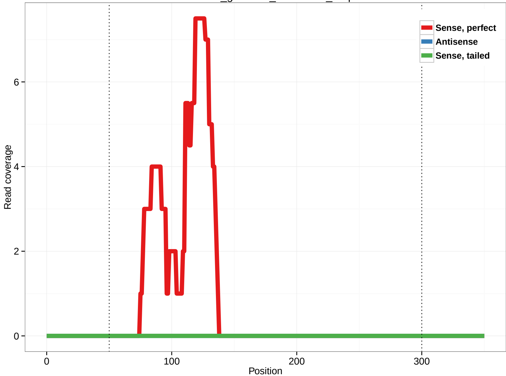
rheMac3_genscan_chr9.1992_1.5p
