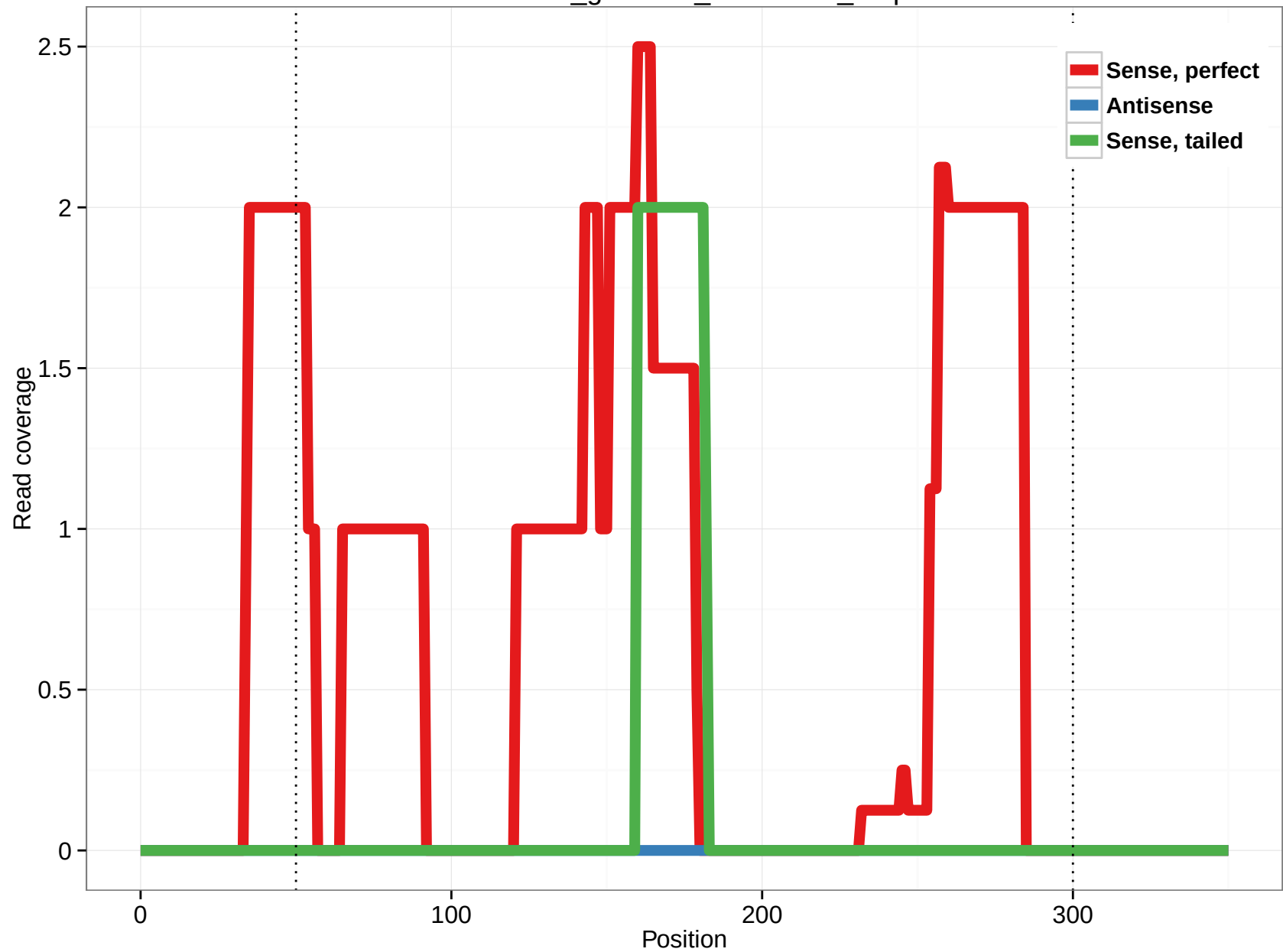
rheMac3_genscan_chr9.1942_2.3p
