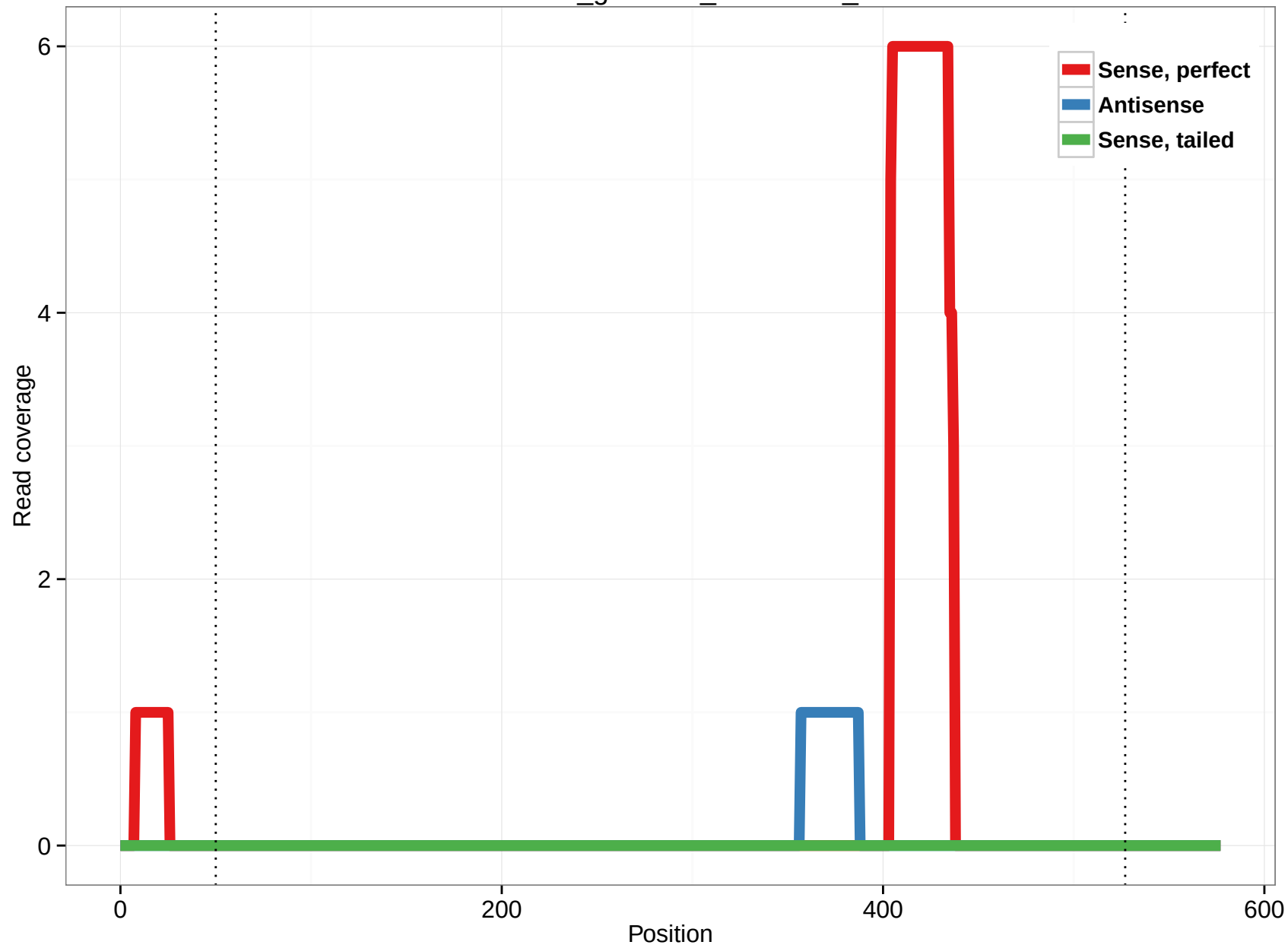
rheMac3_genscan_chr9.1931_2
