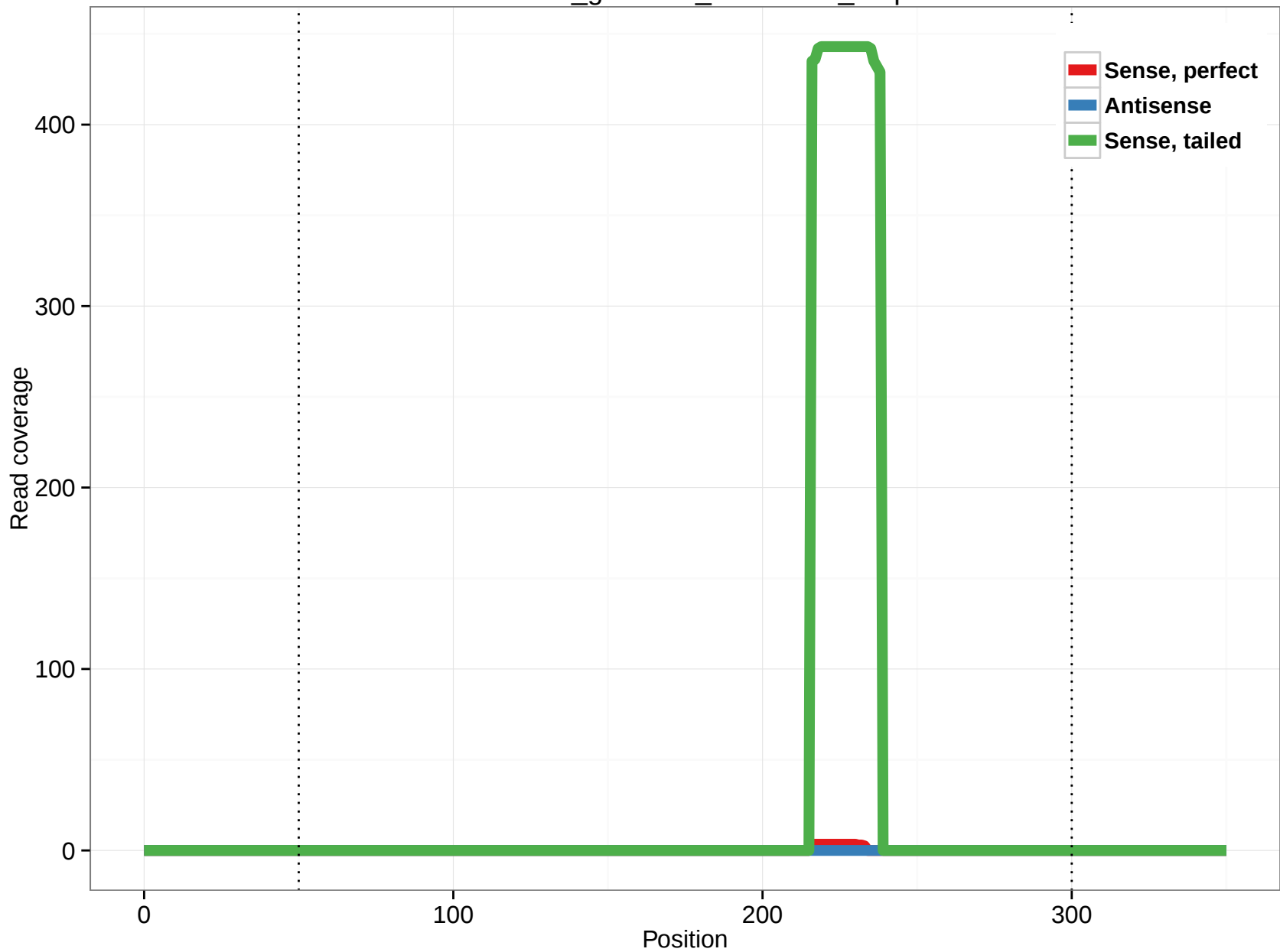
rheMac3_genscan_chr9.1930_8.5p
