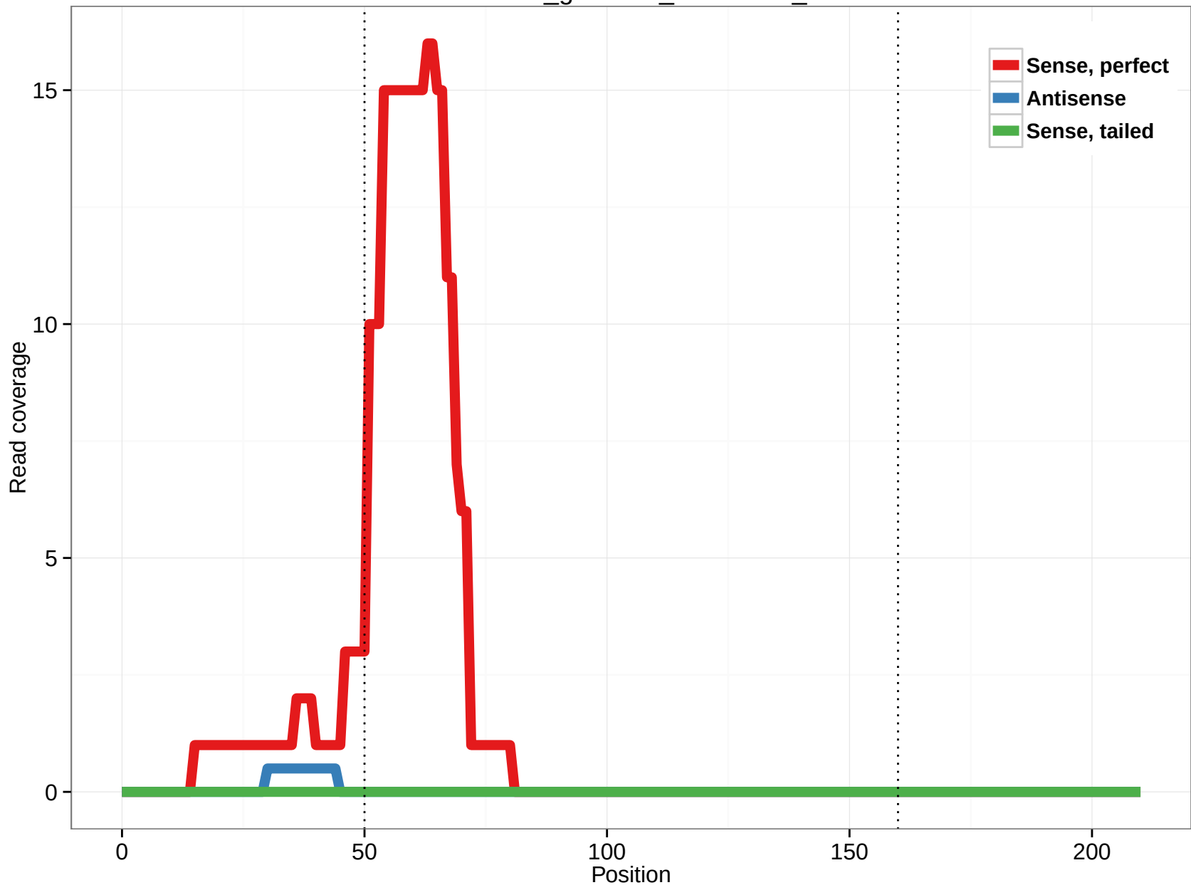
rheMac3_genscan_chr9.1862_1
