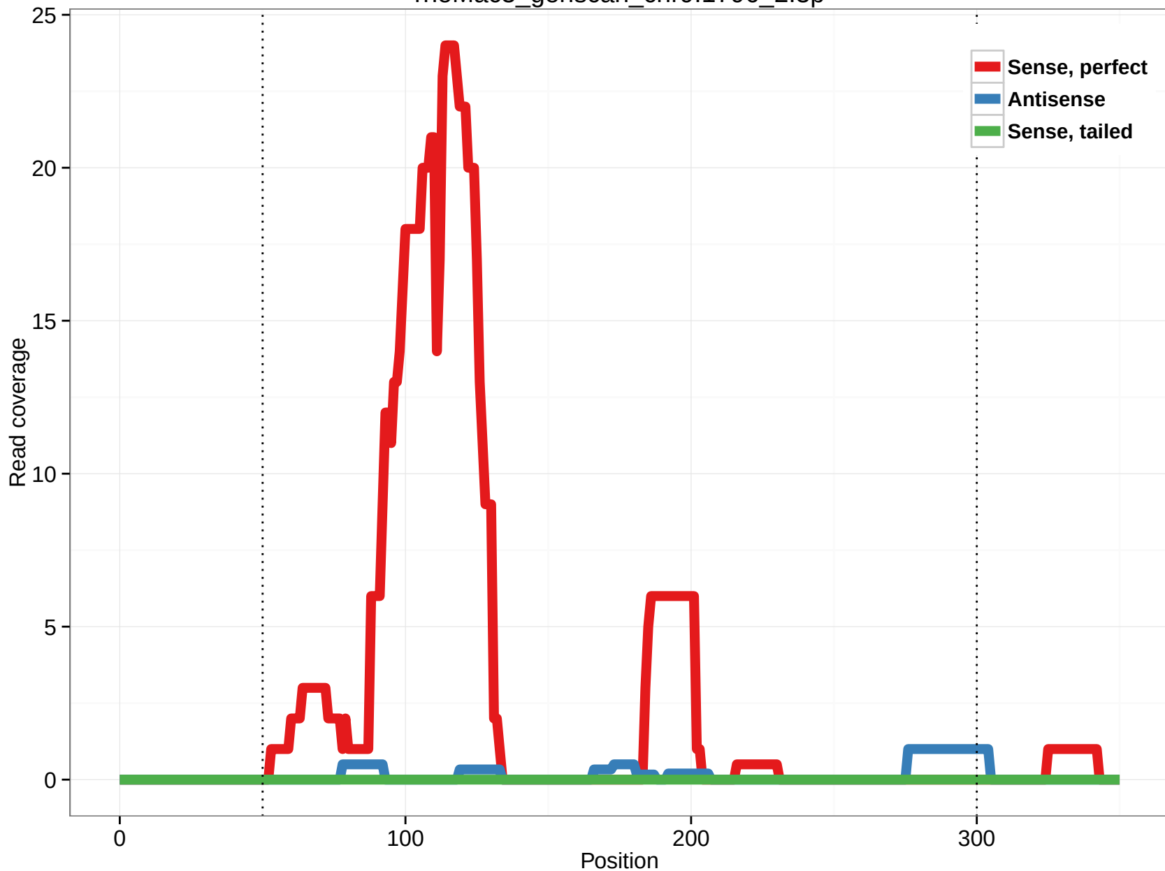
rheMac3_genscan_chr9.1796_2.3p
