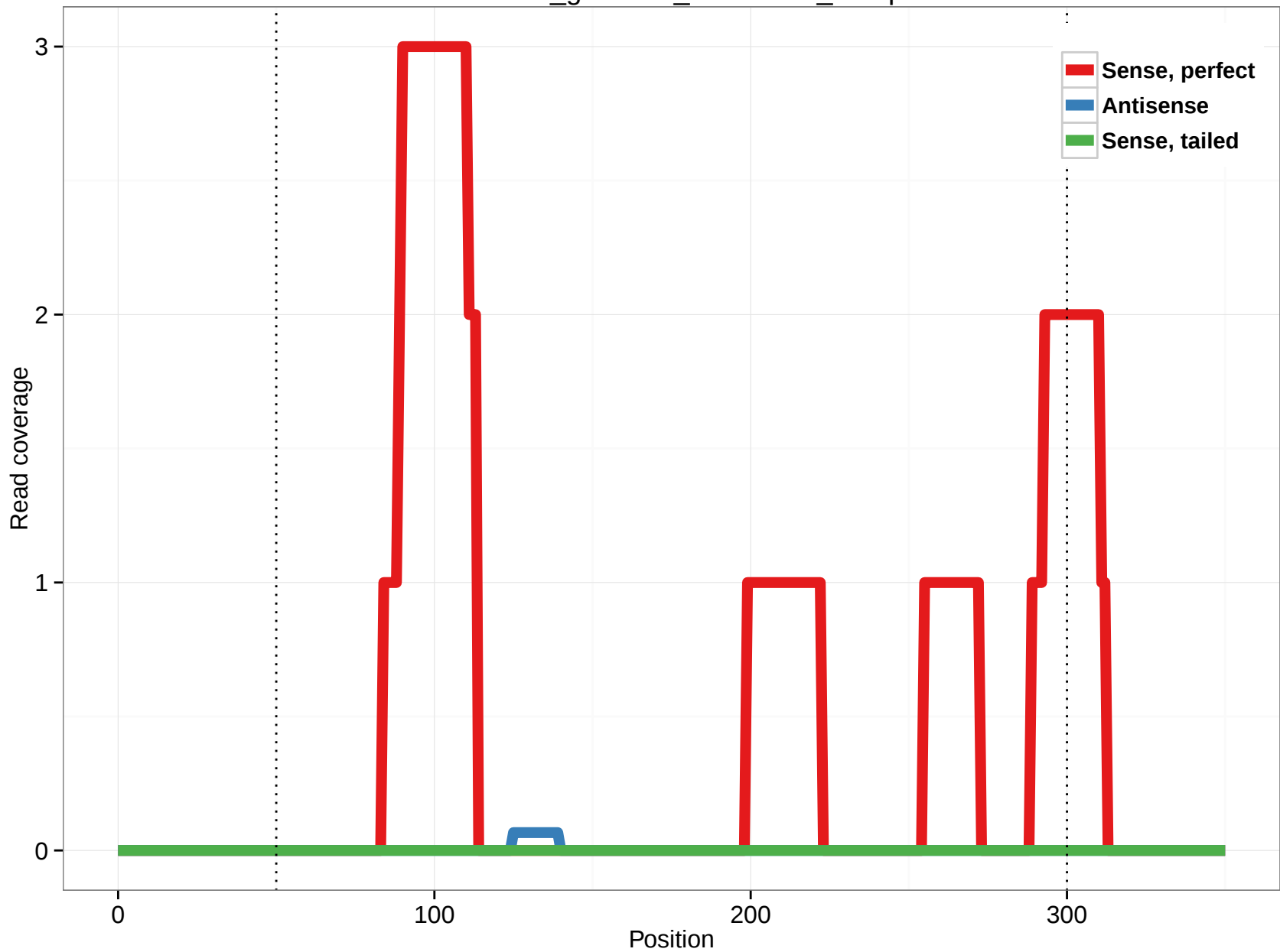
rheMac3_genscan_chr9.1792_27.5p
