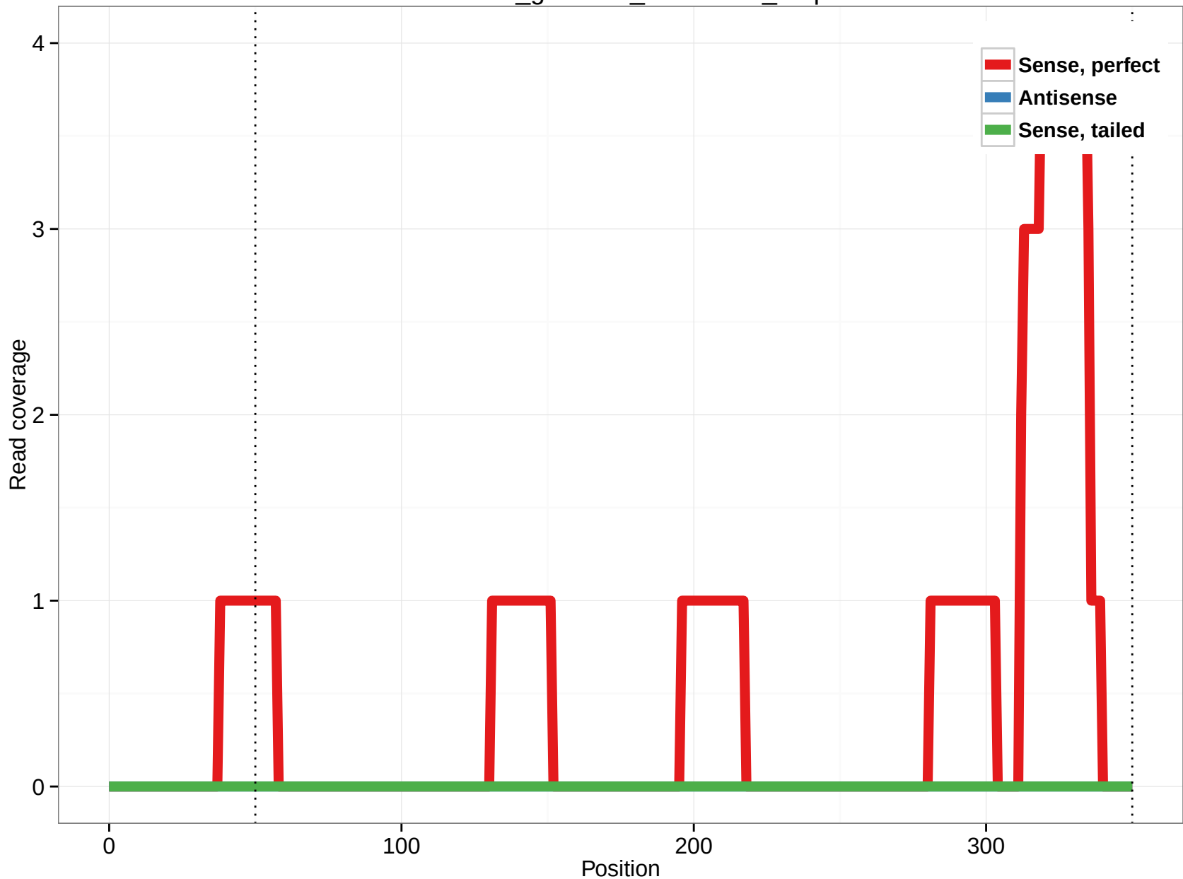
rheMac3_genscan_chr9.1735_9.5p
