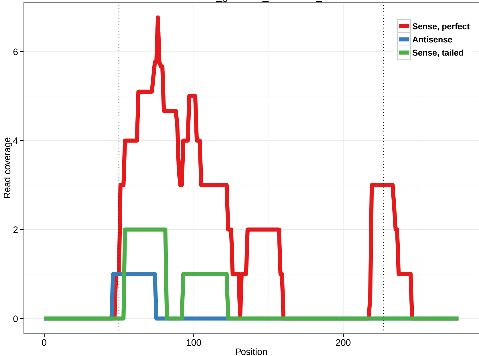
rheMac3_genscan_chr9.1655_4
