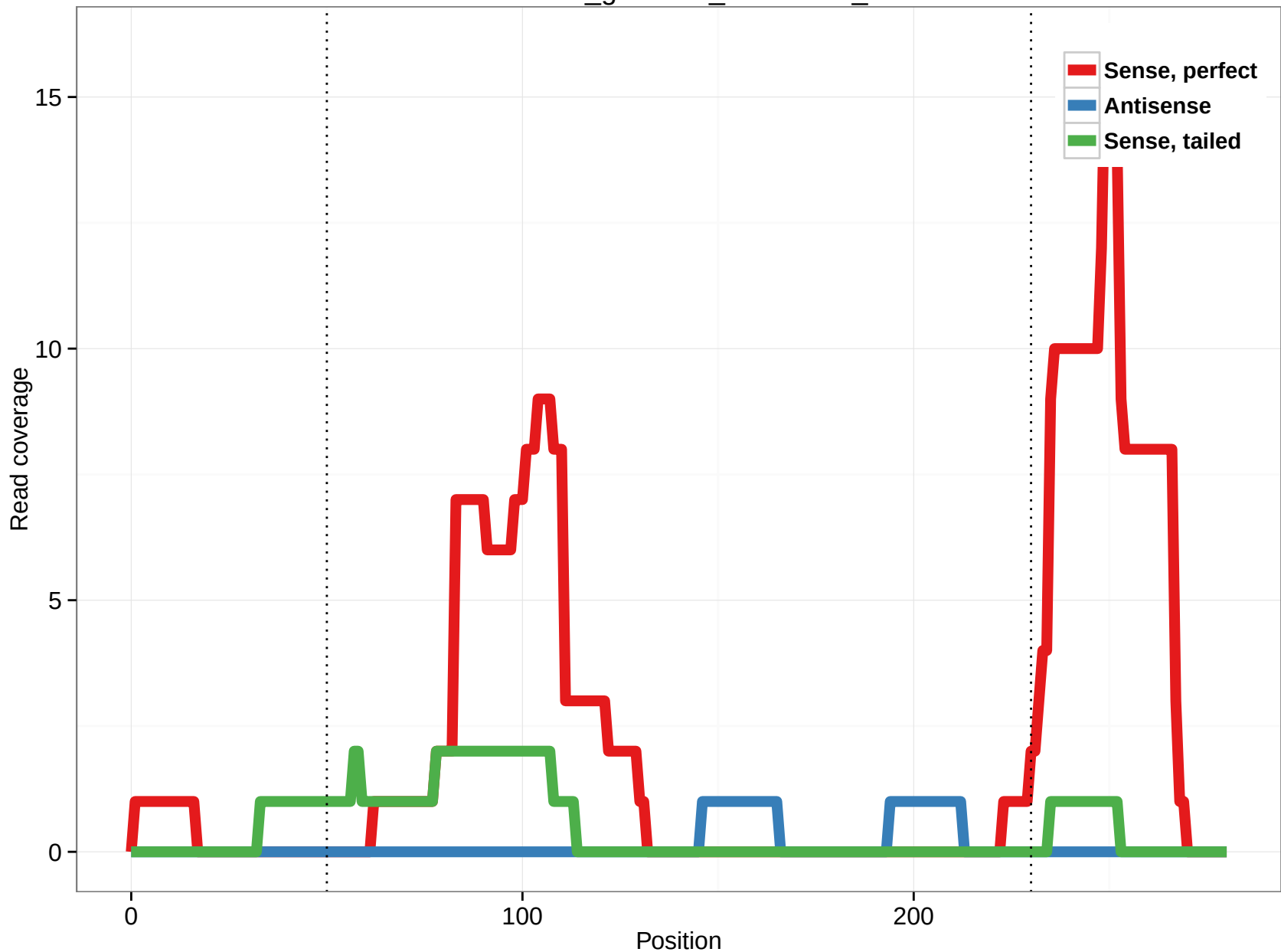
rheMac3_genscan_chr9.1655_3
