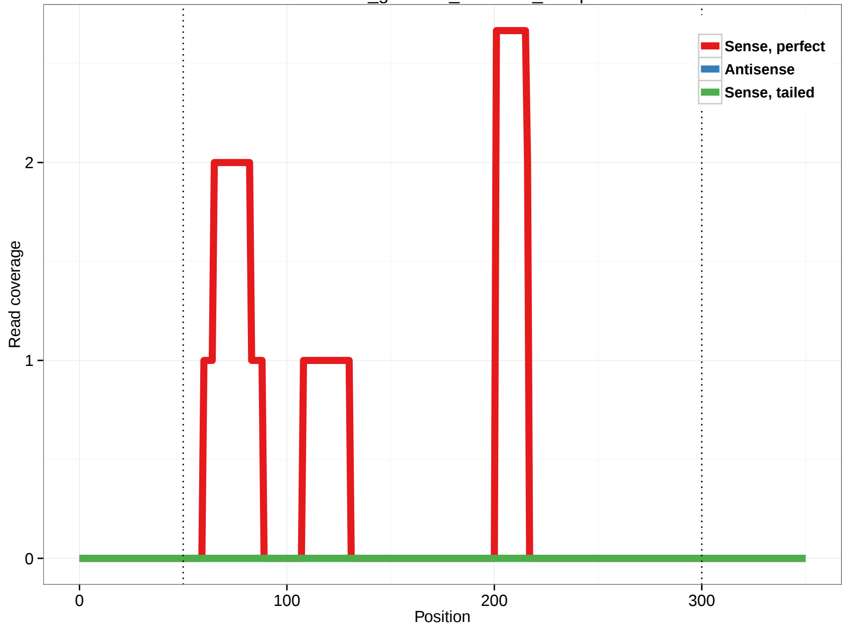
rheMac3_genscan_chr9.162_11.3p
