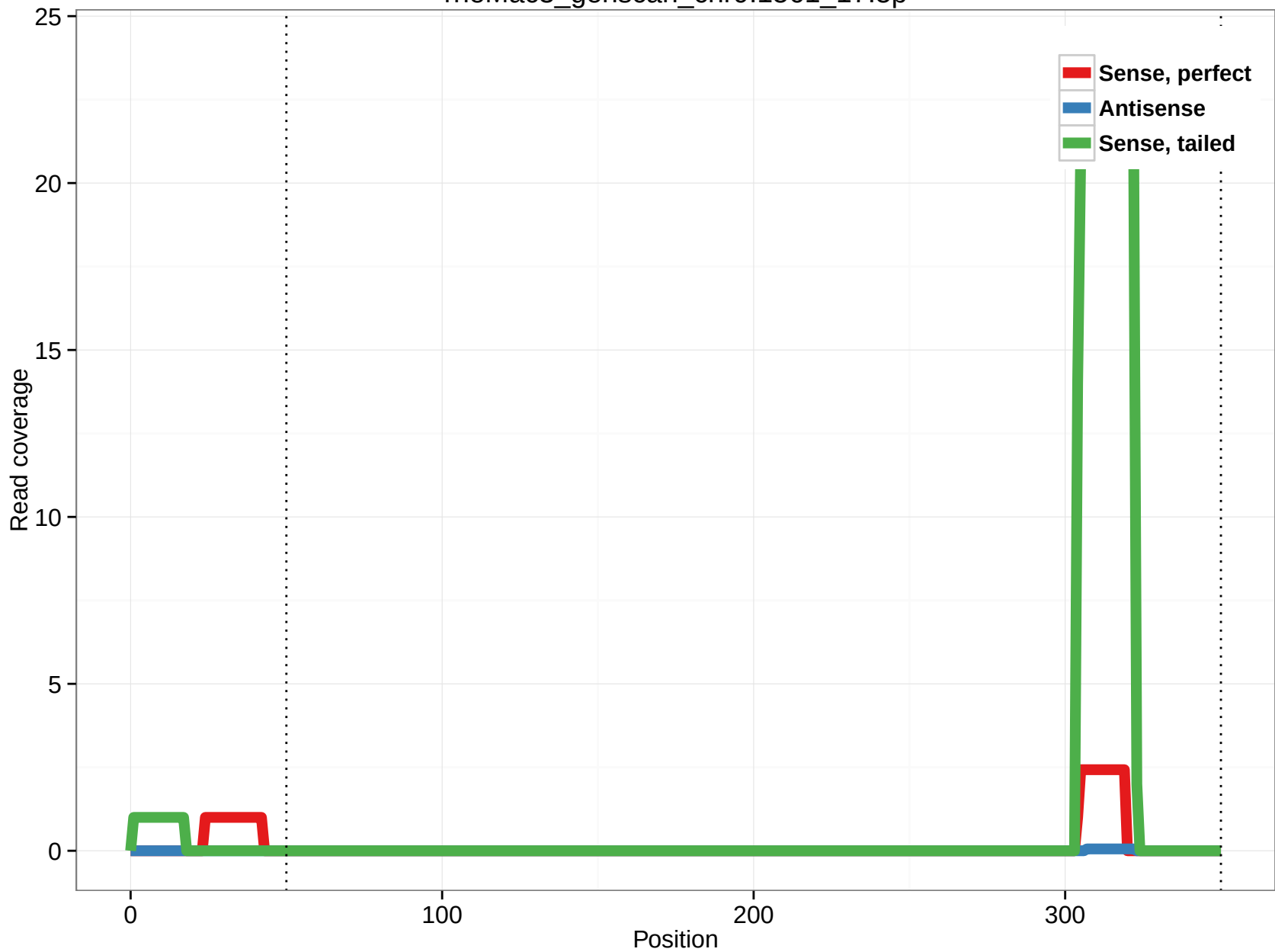
rheMac3_genscan_chr9.1561_17.5p
