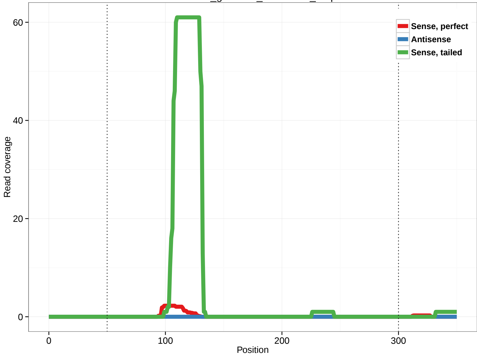
rheMac3_genscan_chr9.1450_3.3p
