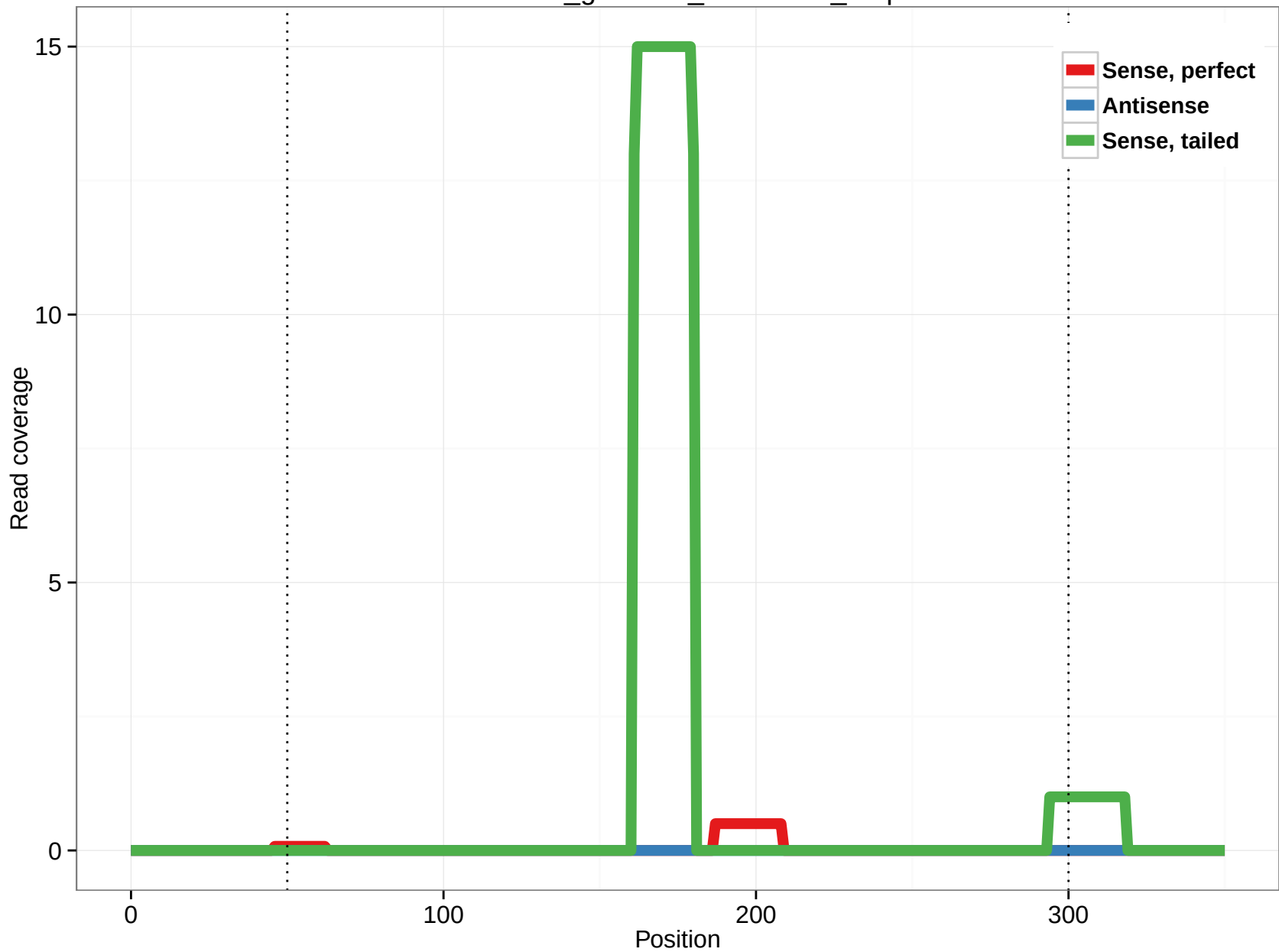
rheMac3_genscan_chr9.1438_8.5p
