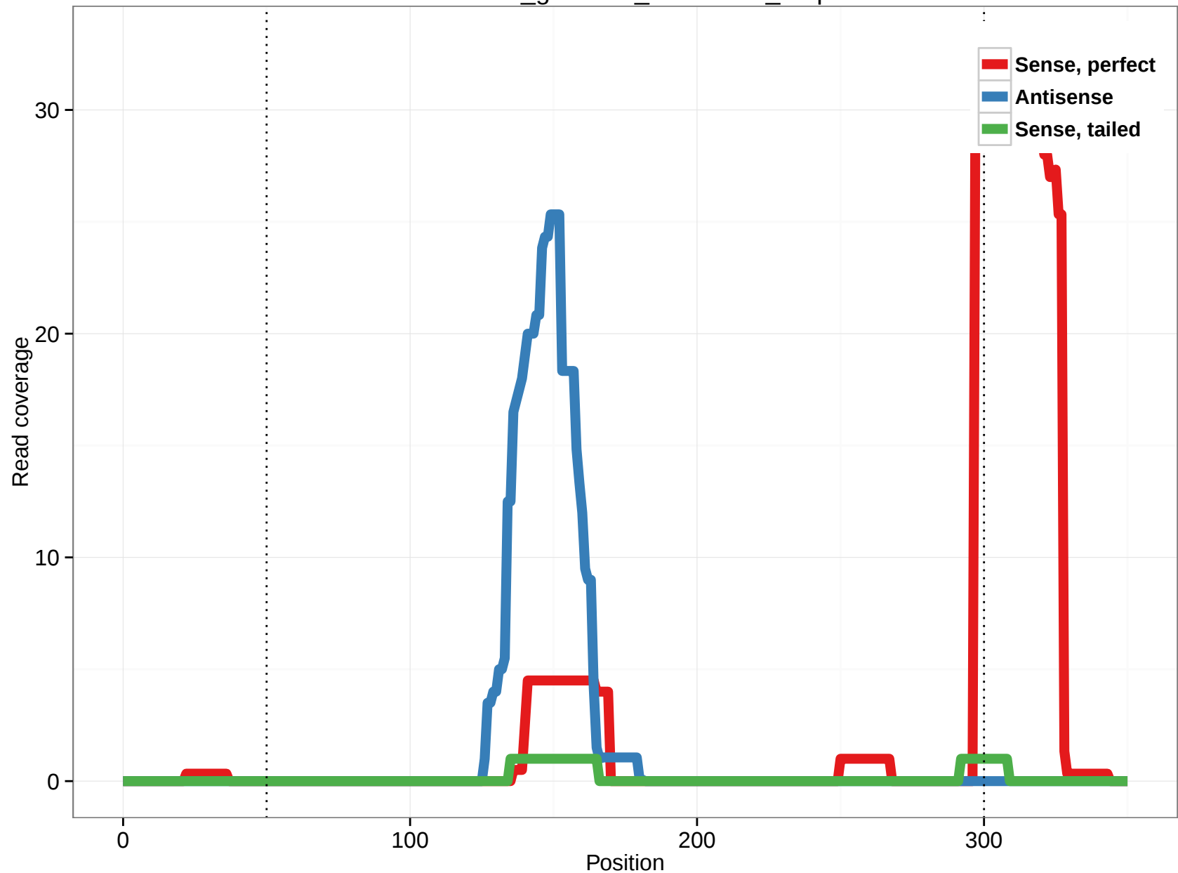
rheMac3_genscan_chr9.1406_7.3p
