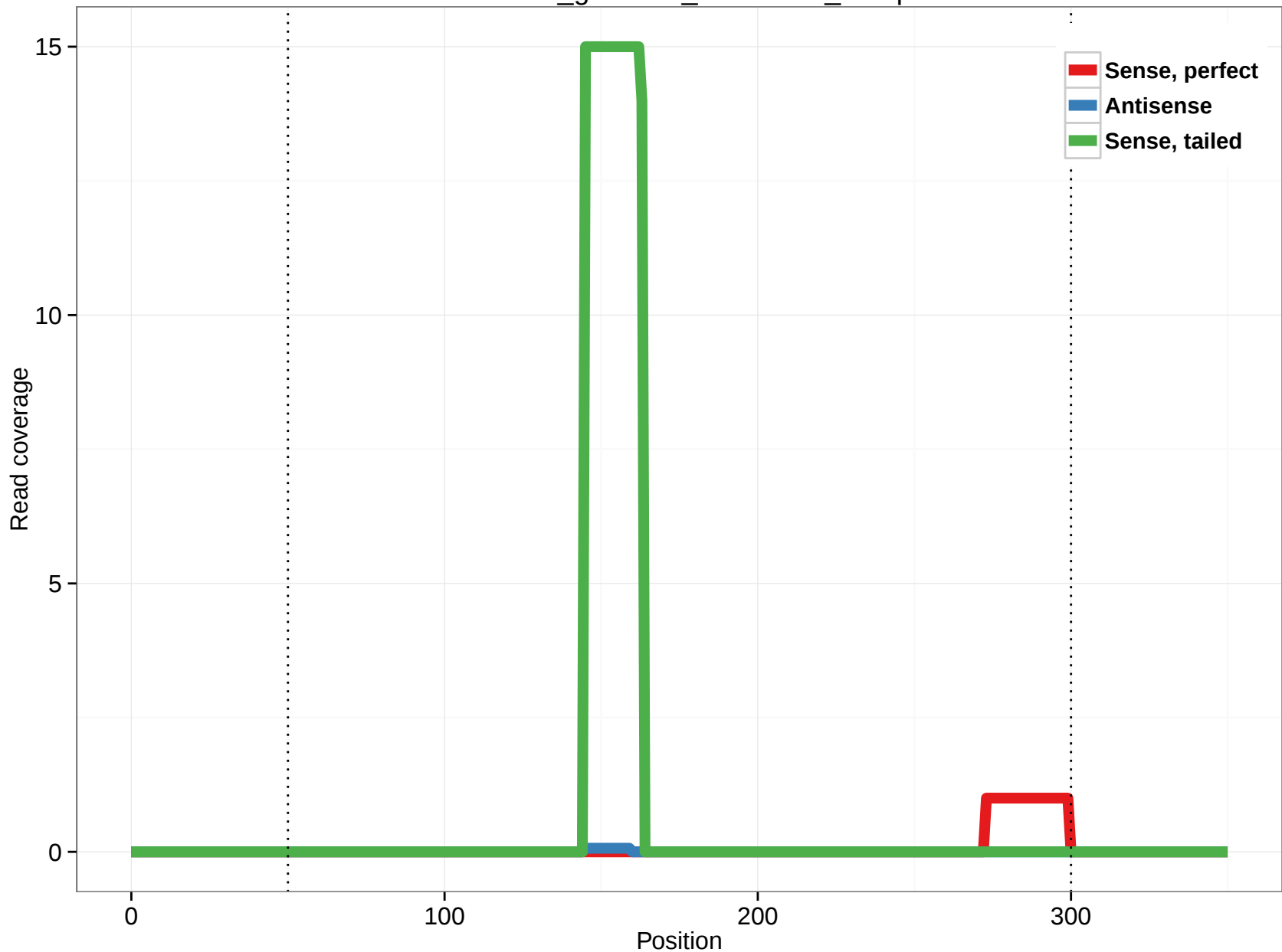
rheMac3_genscan_chr9.1327_14.3p
