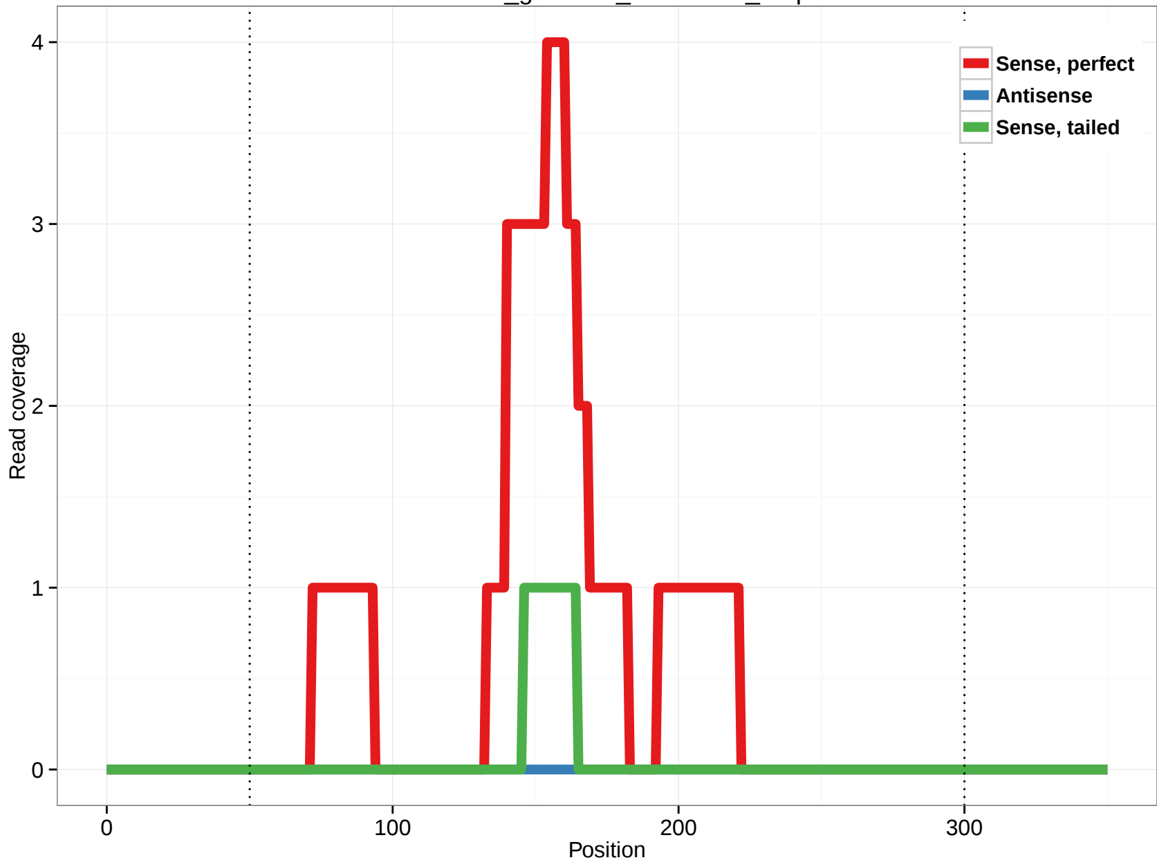
rheMac3_genscan_chr9.1310_2.5p
