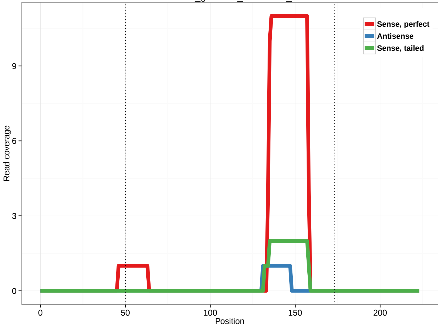
rheMac3_genscan_chr9.1309_20
