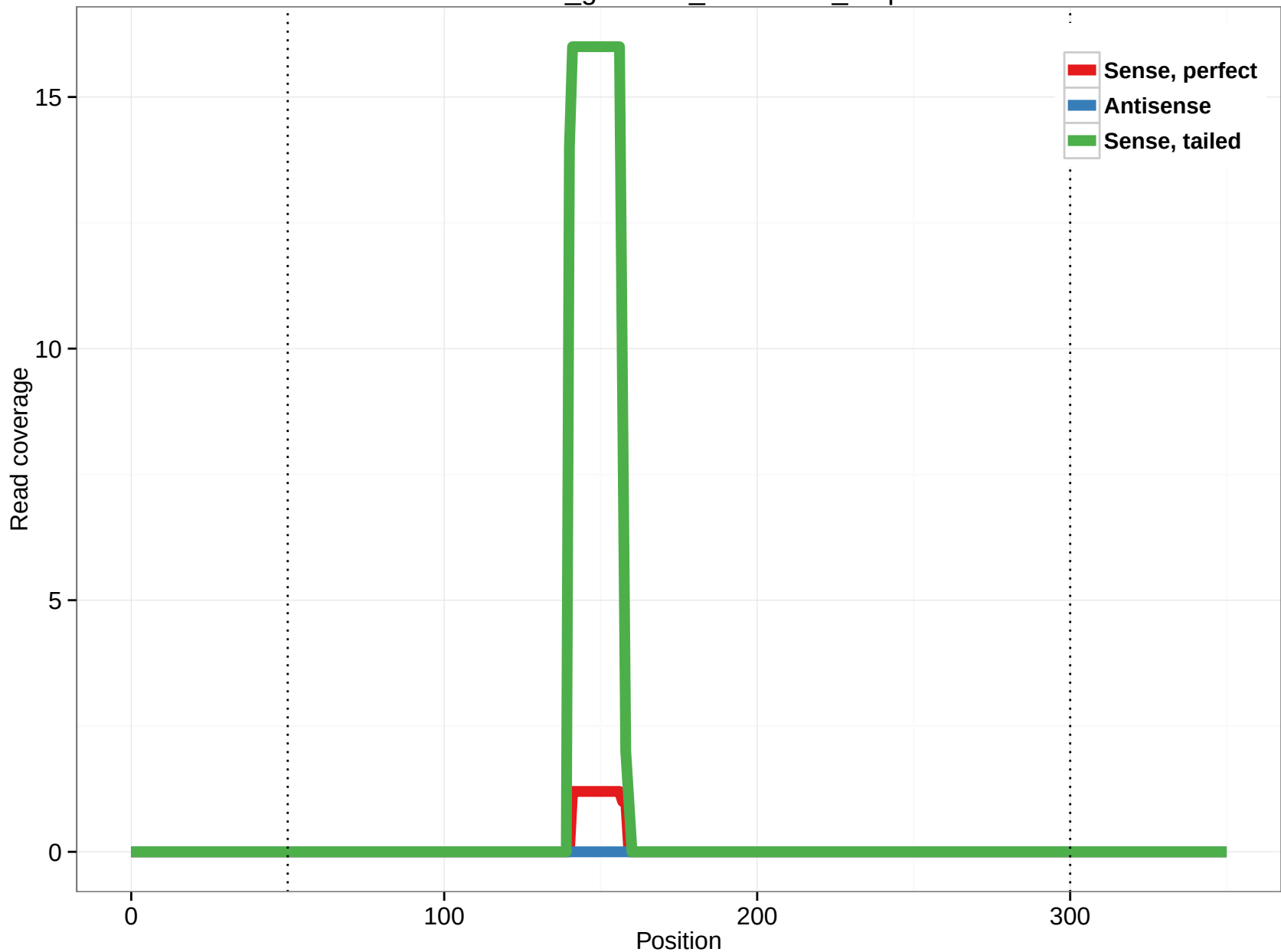
rheMac3_genscan_chr9.1304_0.3p
