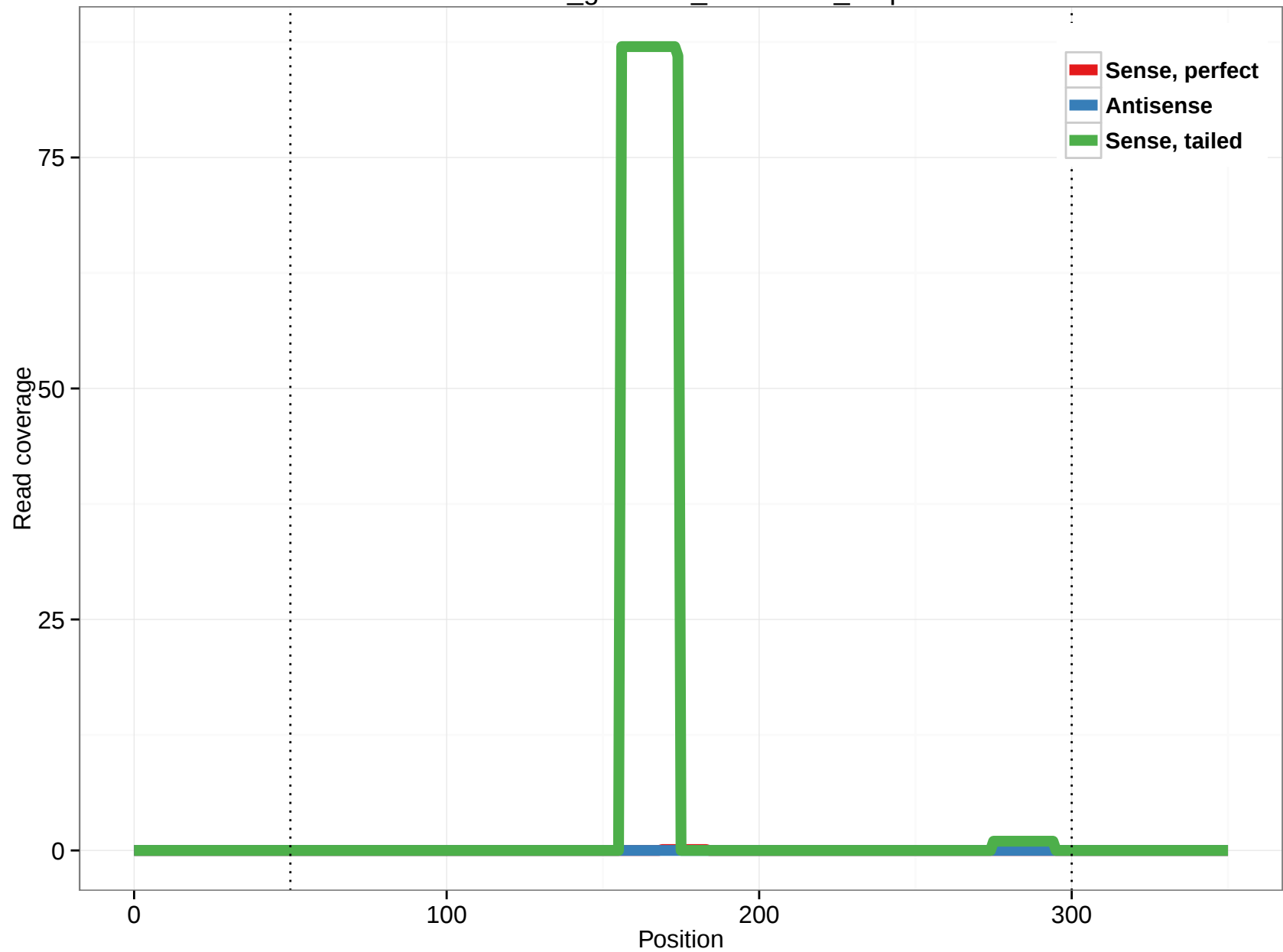
rheMac3_genscan_chr9.1299_1.5p
