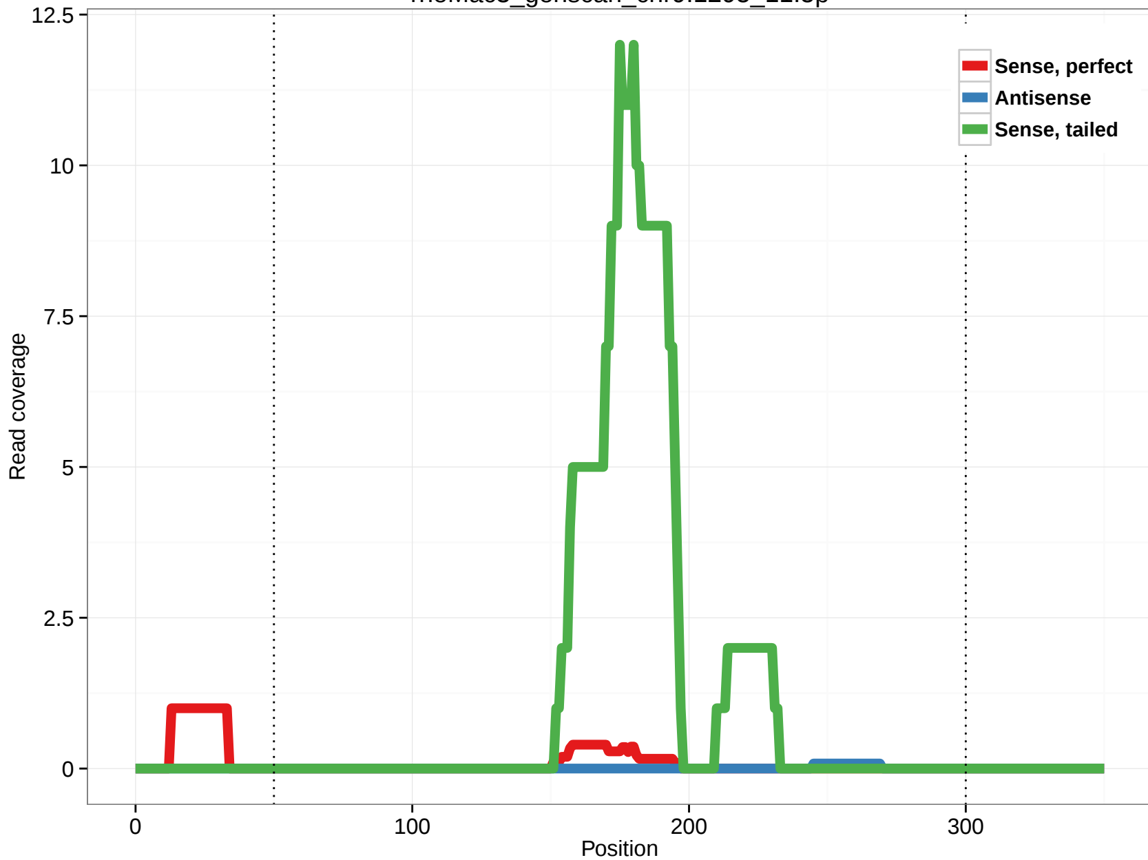
rheMac3_genscan_chr9.1295_11.5p
