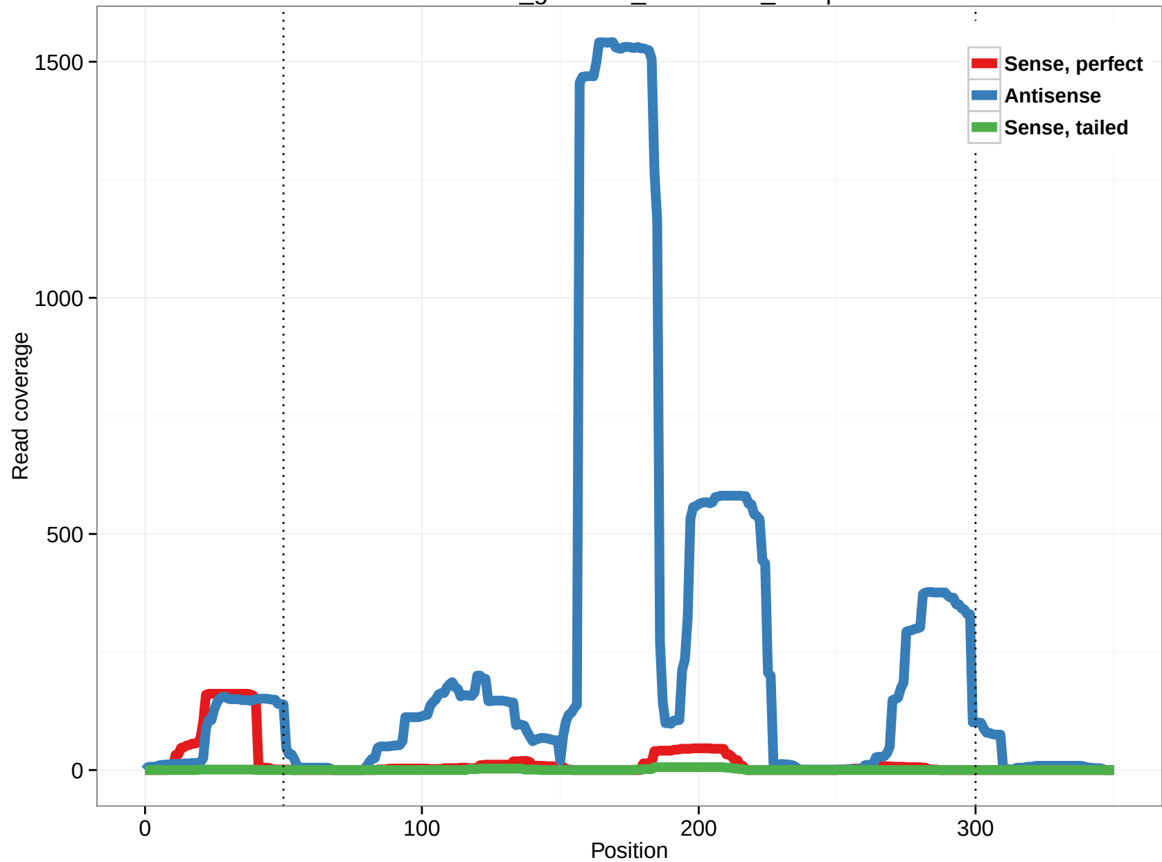
rheMac3_genscan_chr9.1224_40.3p
