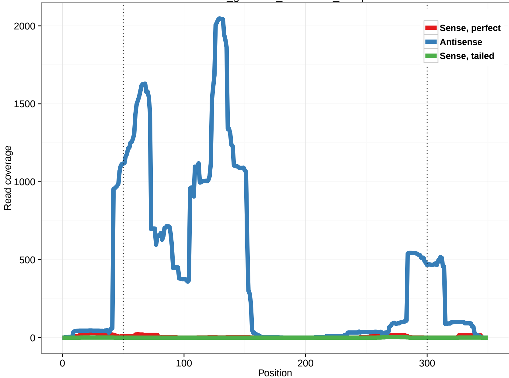
rheMac3_genscan_chr9.1224_39.5p
