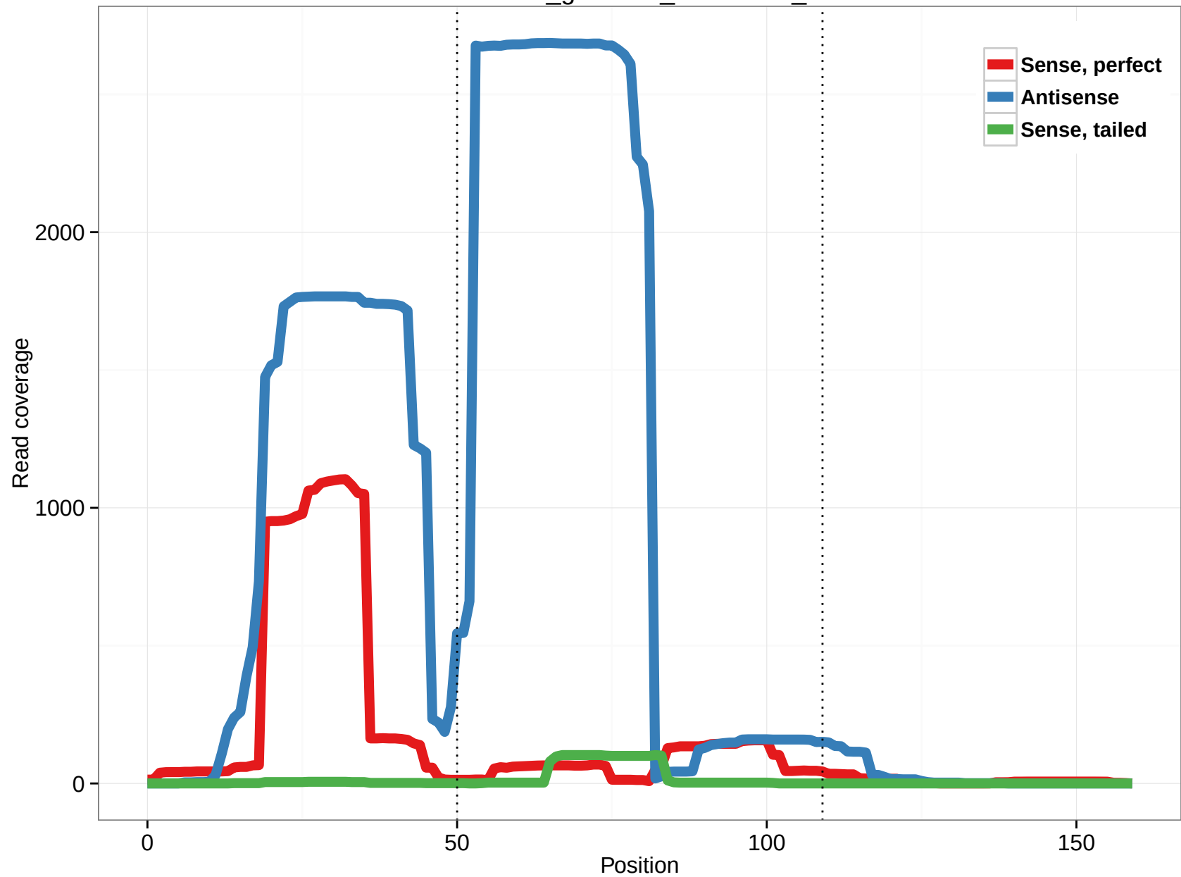
rheMac3_genscan_chr9.1224_35
