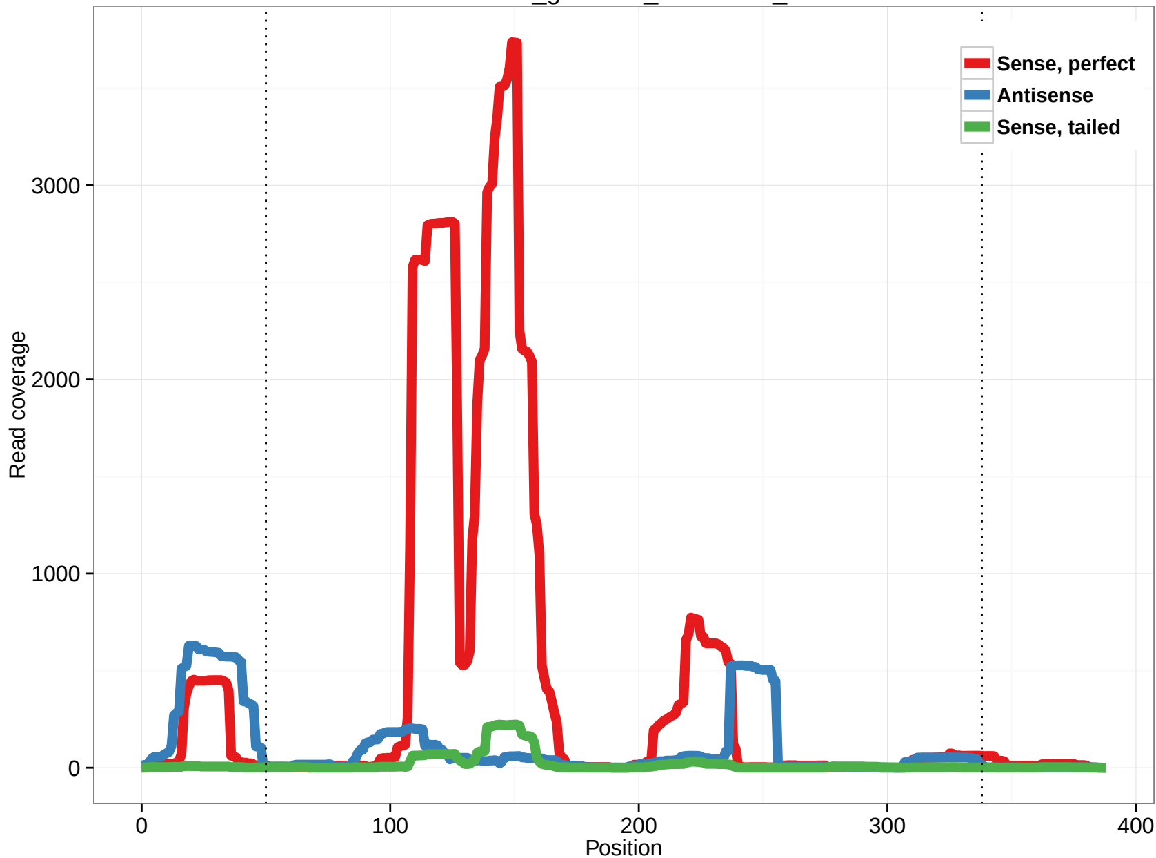
rheMac3_genscan_chr9.1224_34
