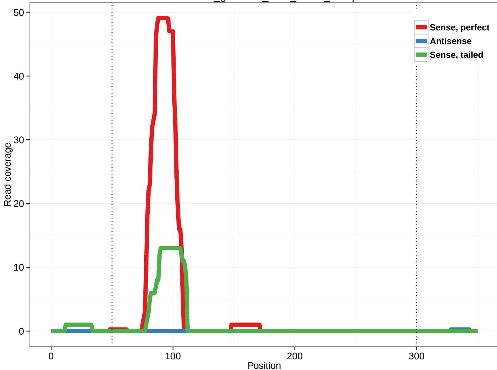
rheMac3_genscan_chr8_87.17_46.5p
