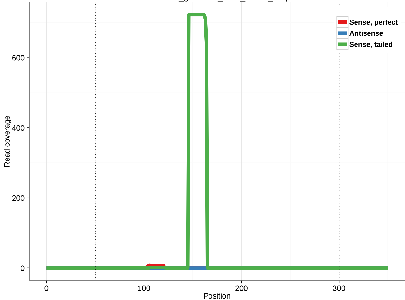
rheMac3_genscan_chr8_87.11_0.3p
