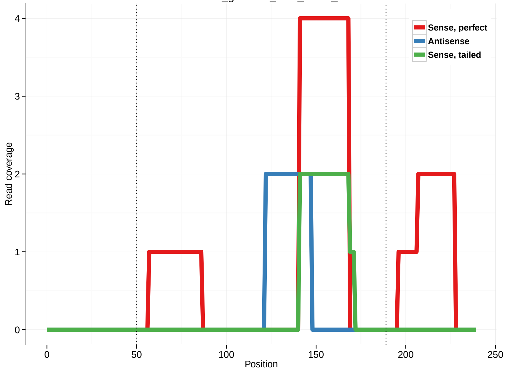
rheMac3_genscan_chr8_78.88_1
