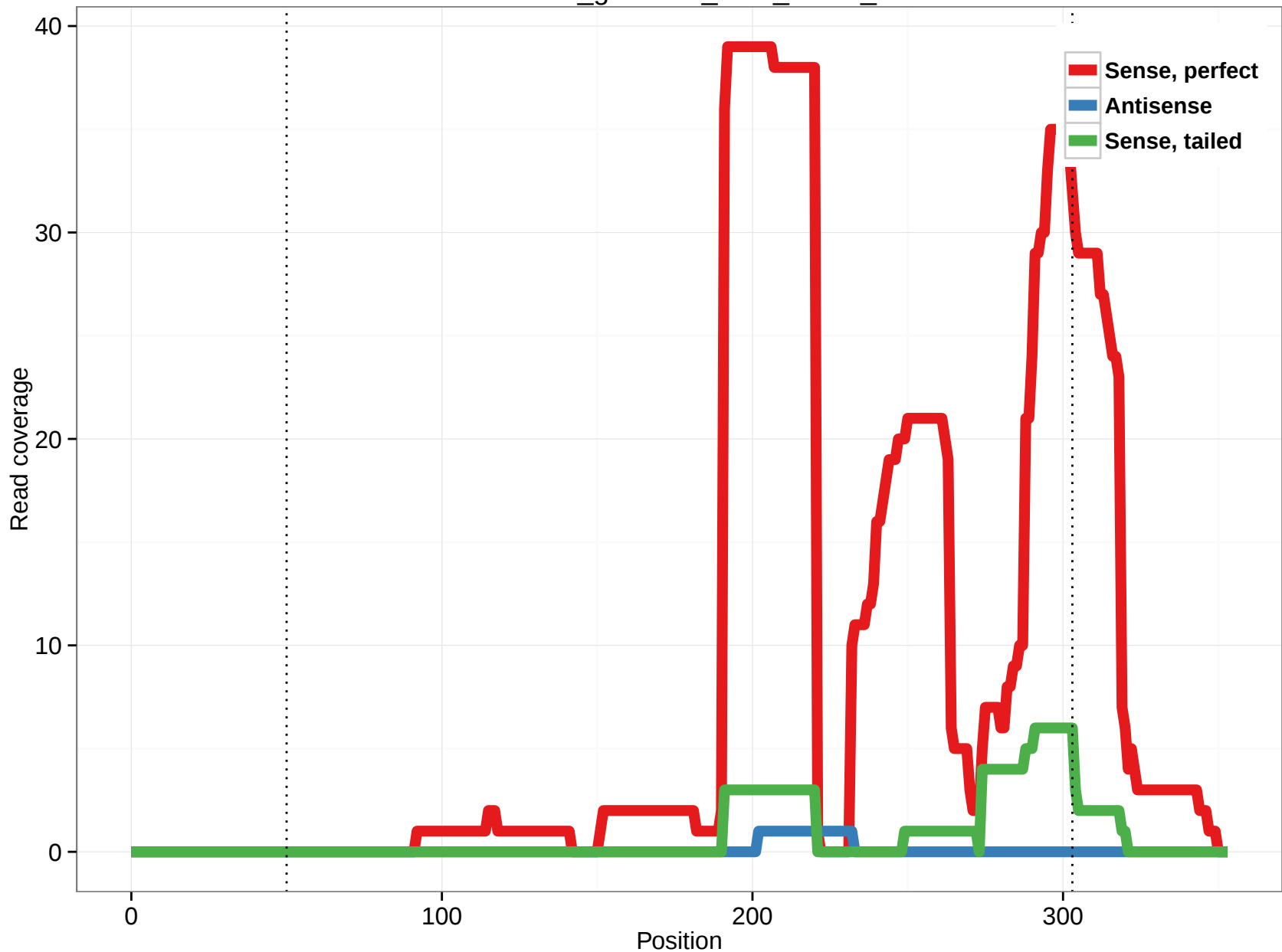
rheMac3_genscan_chr8_78.72_6
