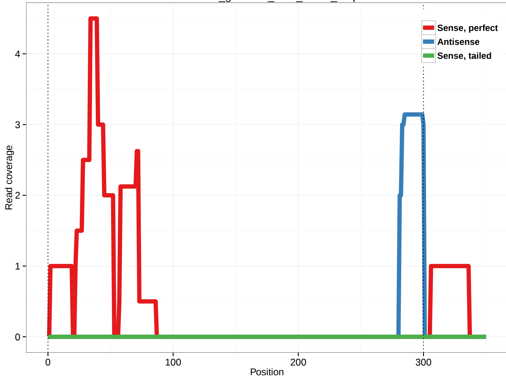
rheMac3_genscan_chr8_78.52_0.3p
