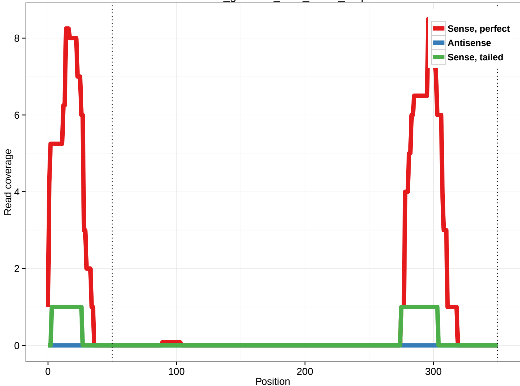
rheMac3_genscan_chr8_78.51_7.5p
