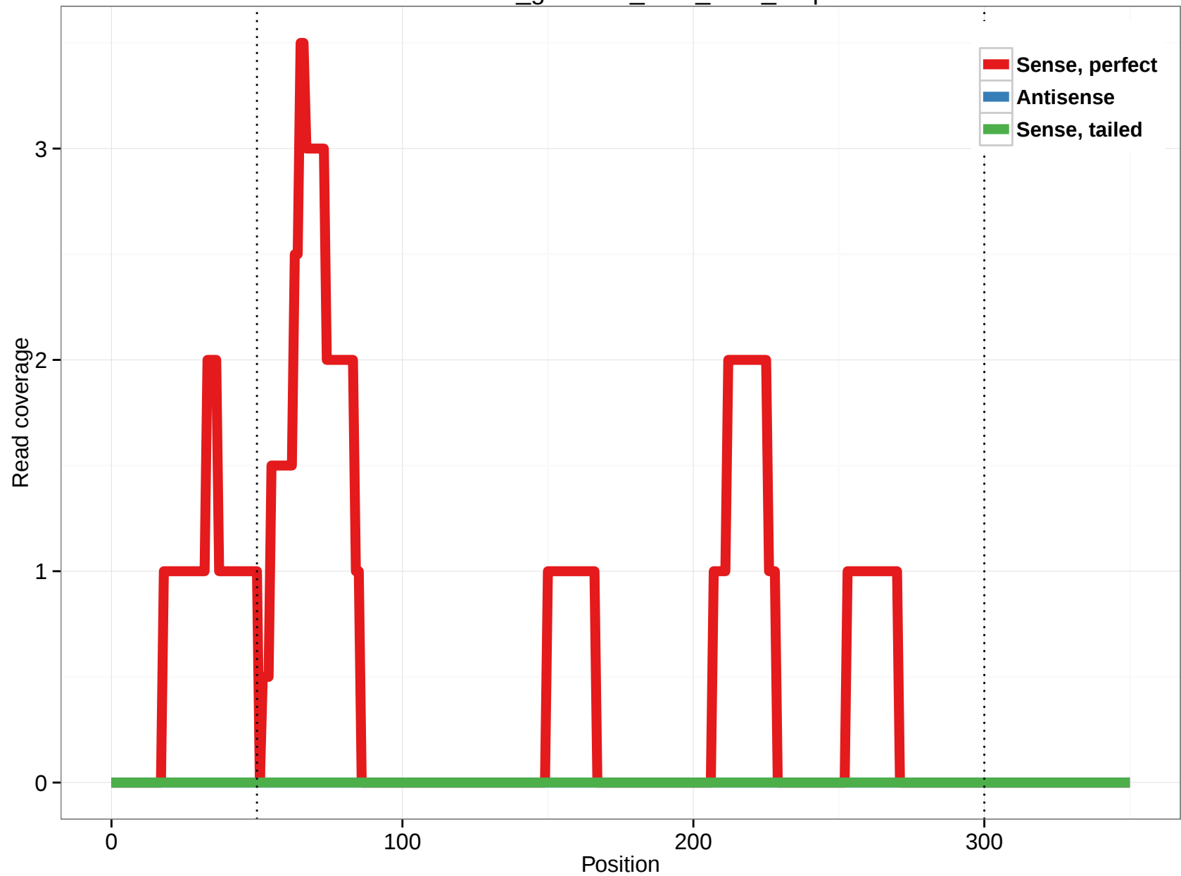
rheMac3_genscan_chr8_78.4_0.3p
