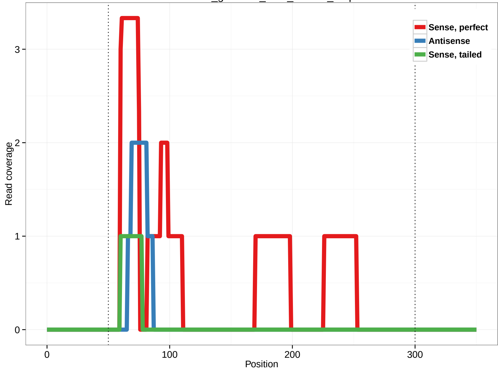
rheMac3_genscan_chr8_78.286_2.5p
