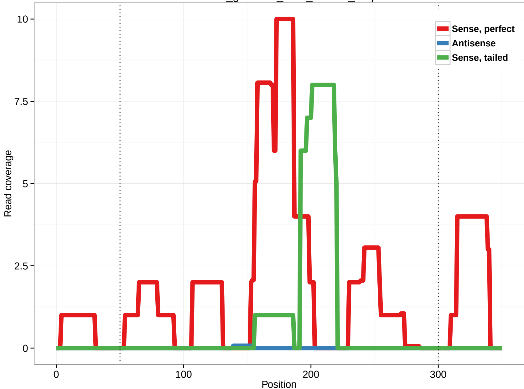
rheMac3_genscan_chr8_78.251_6.5p
