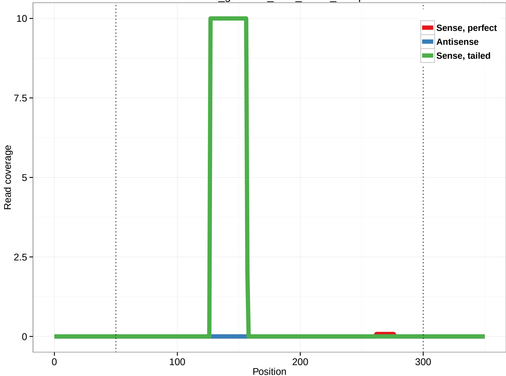
rheMac3_genscan_chr8_78.21_15.3p
