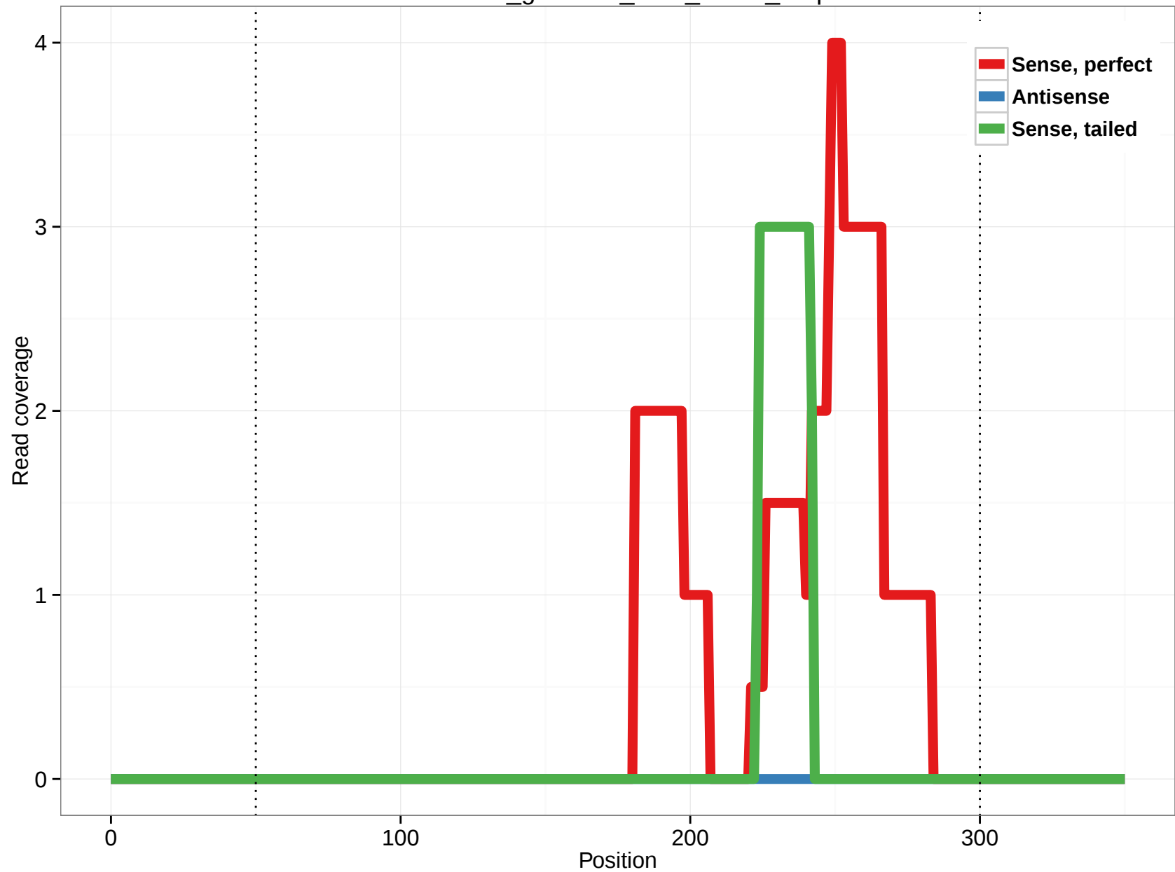
rheMac3_genscan_chr8_78.19_2.3p
