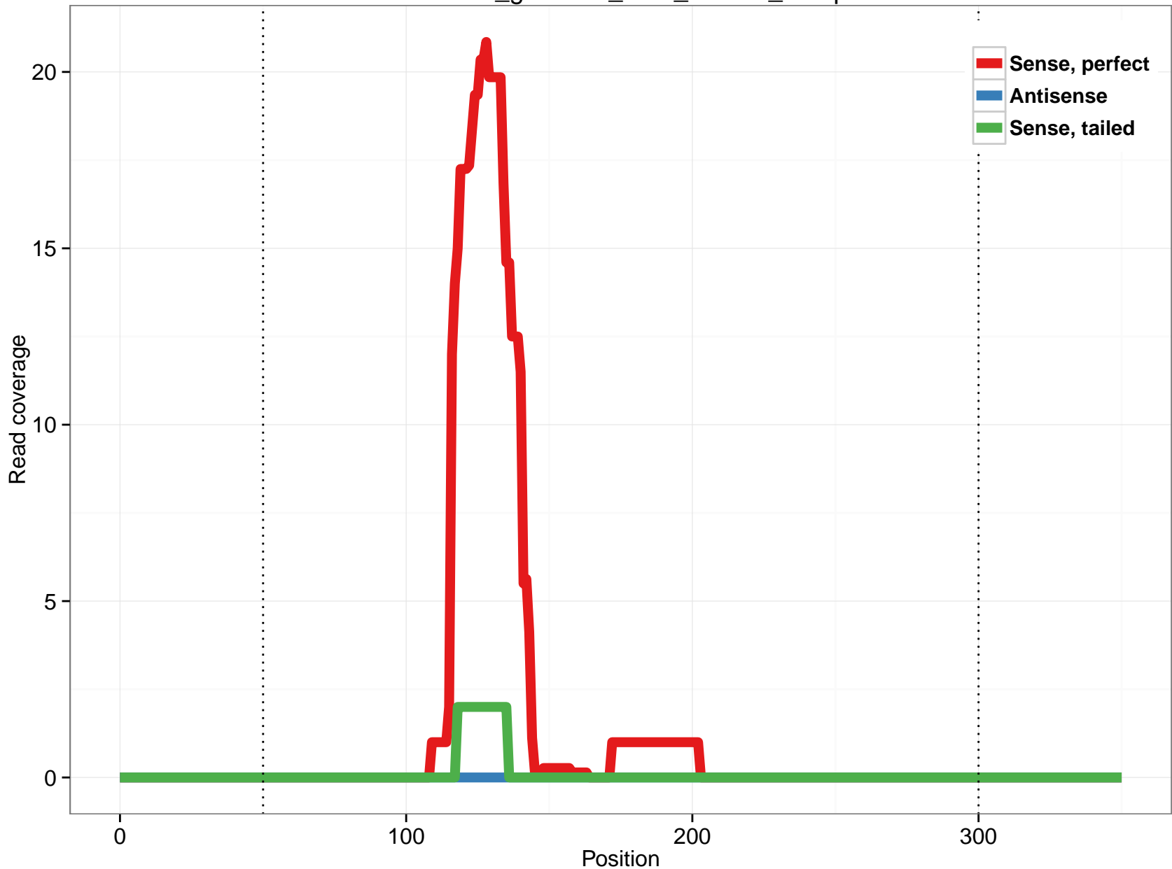
rheMac3_genscan_chr8_78.138_16.5p
