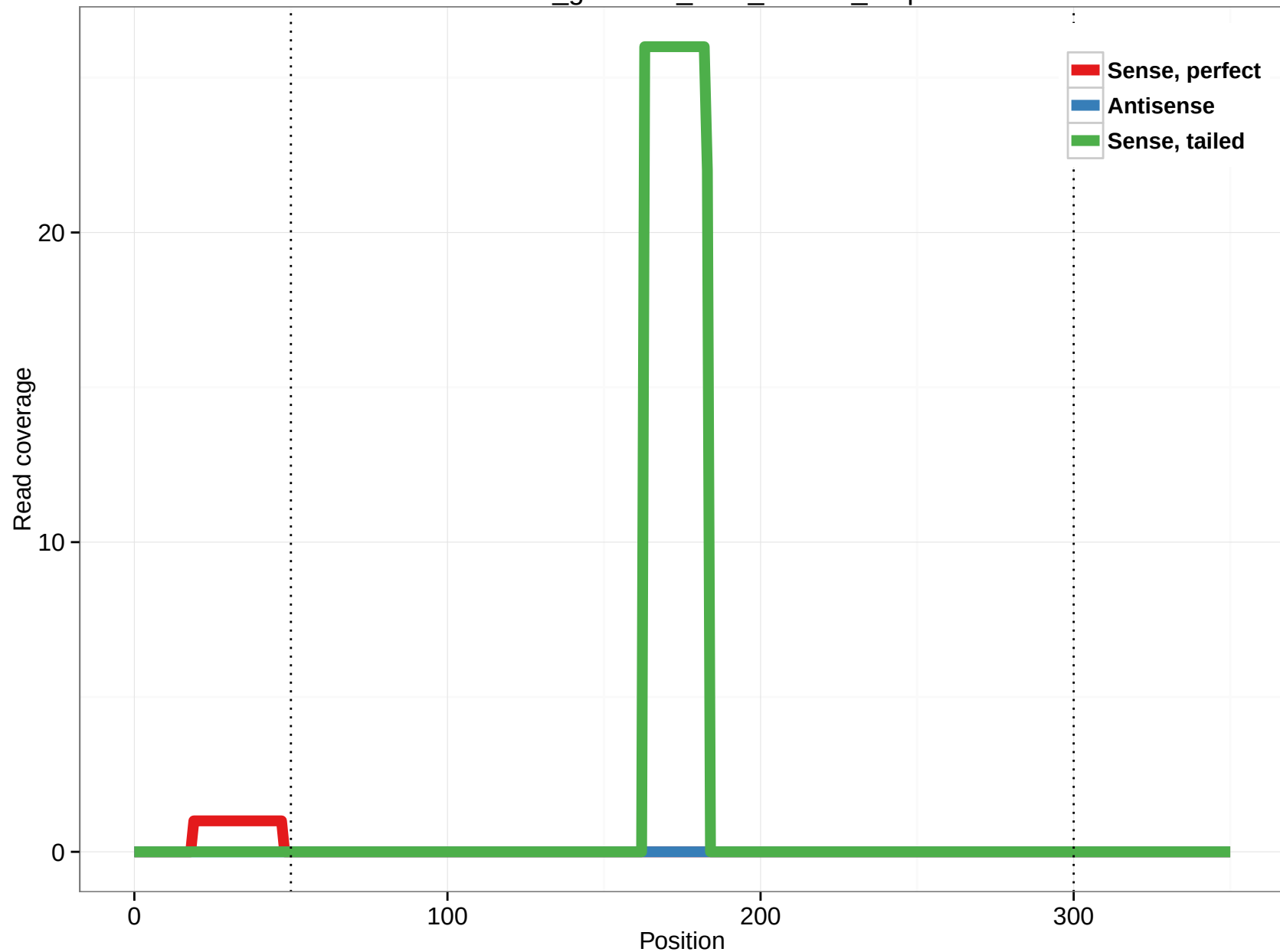
rheMac3_genscan_chr8_78.135_3.5p
