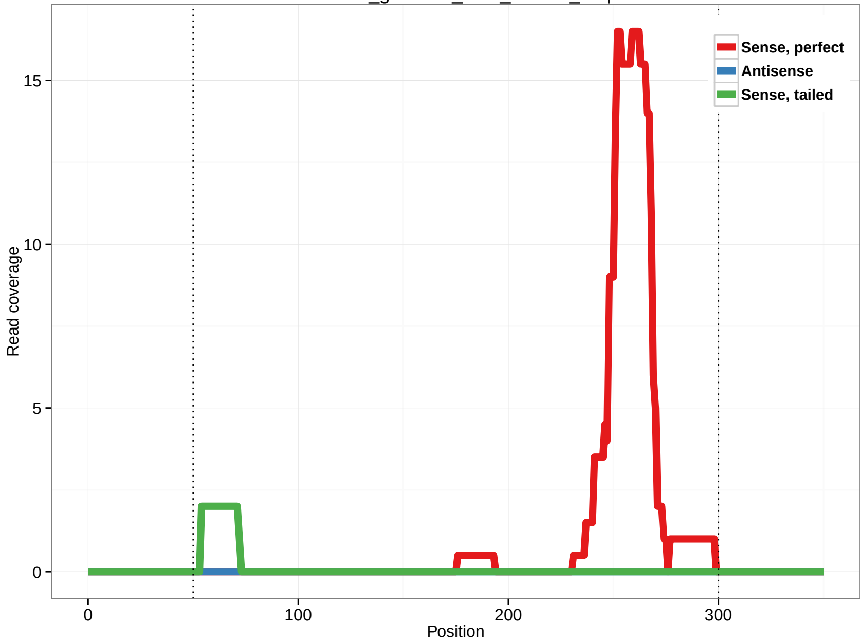
rheMac3_genscan_chr8_78.110_2.5p
