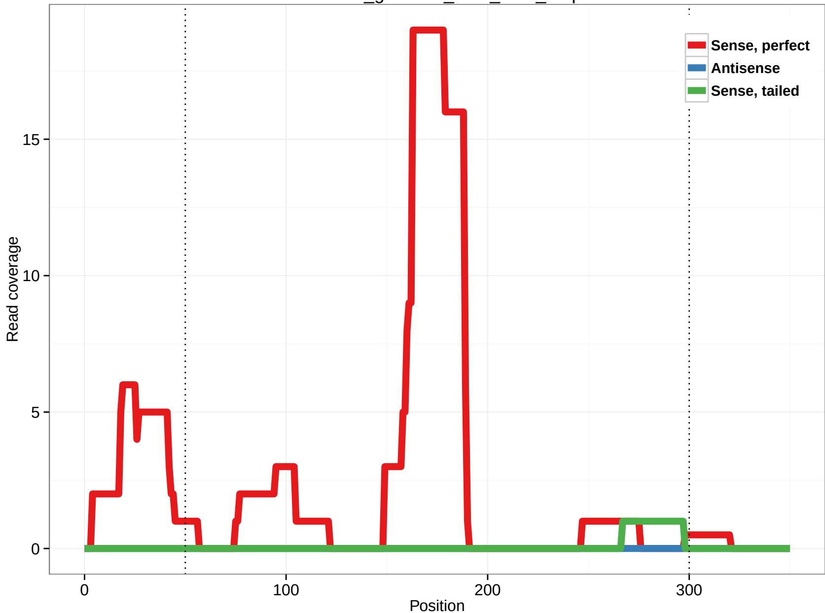
rheMac3_genscan_chr8_73.3_9.5p
