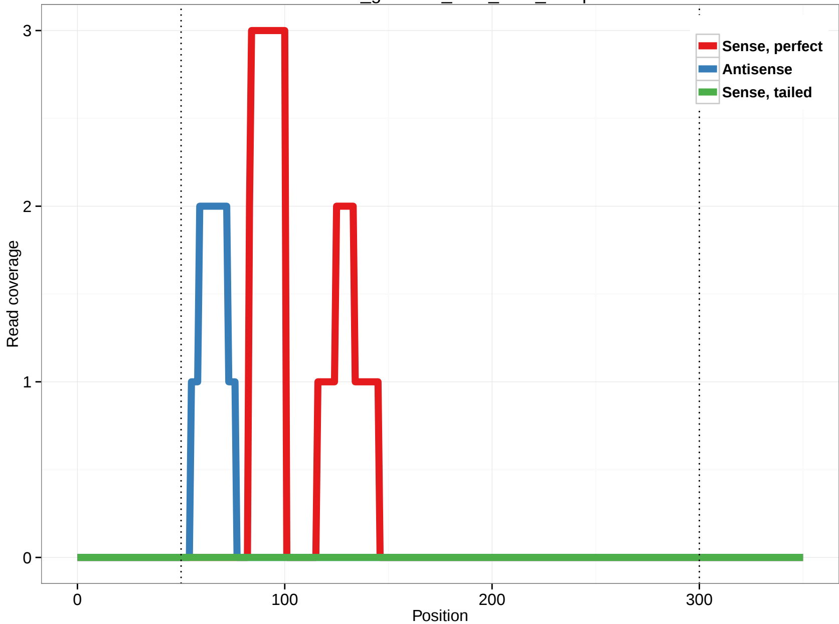
rheMac3_genscan_chr8_72.3_18.5p
