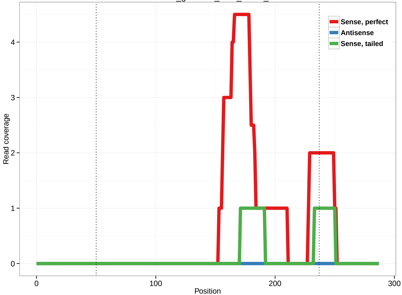
rheMac3_genscan_chr8_67.13_7
