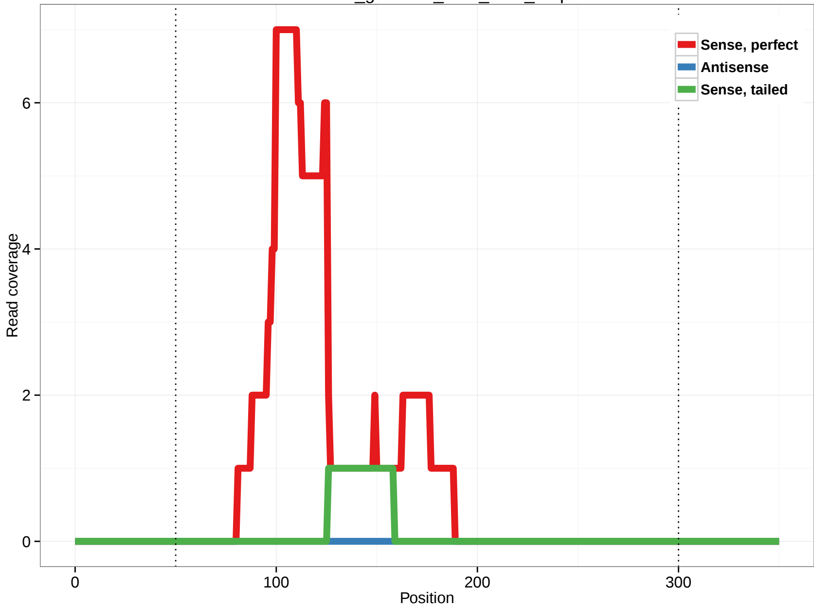
rheMac3_genscan_chr8_54.5_8.3p
