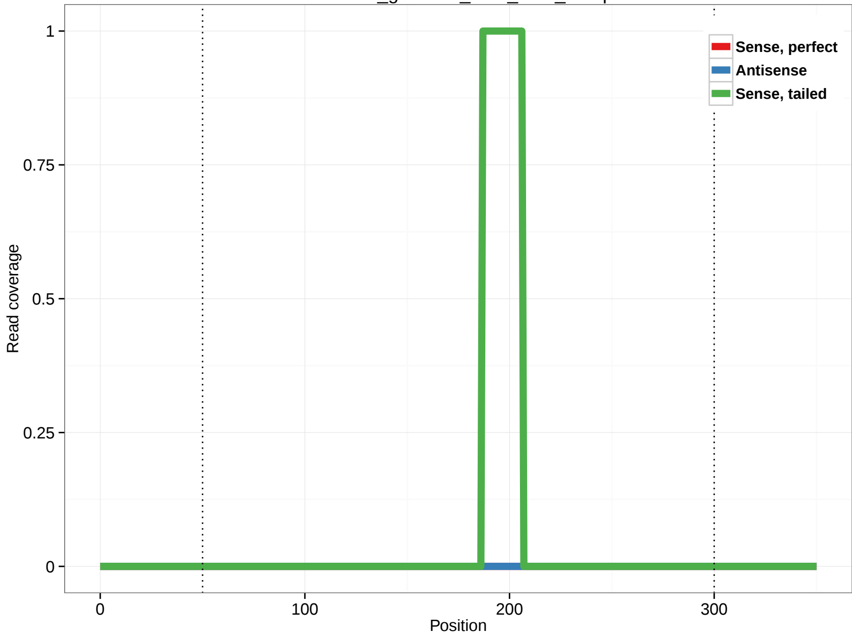
rheMac3_genscan_chr8_54.5_18.3p
