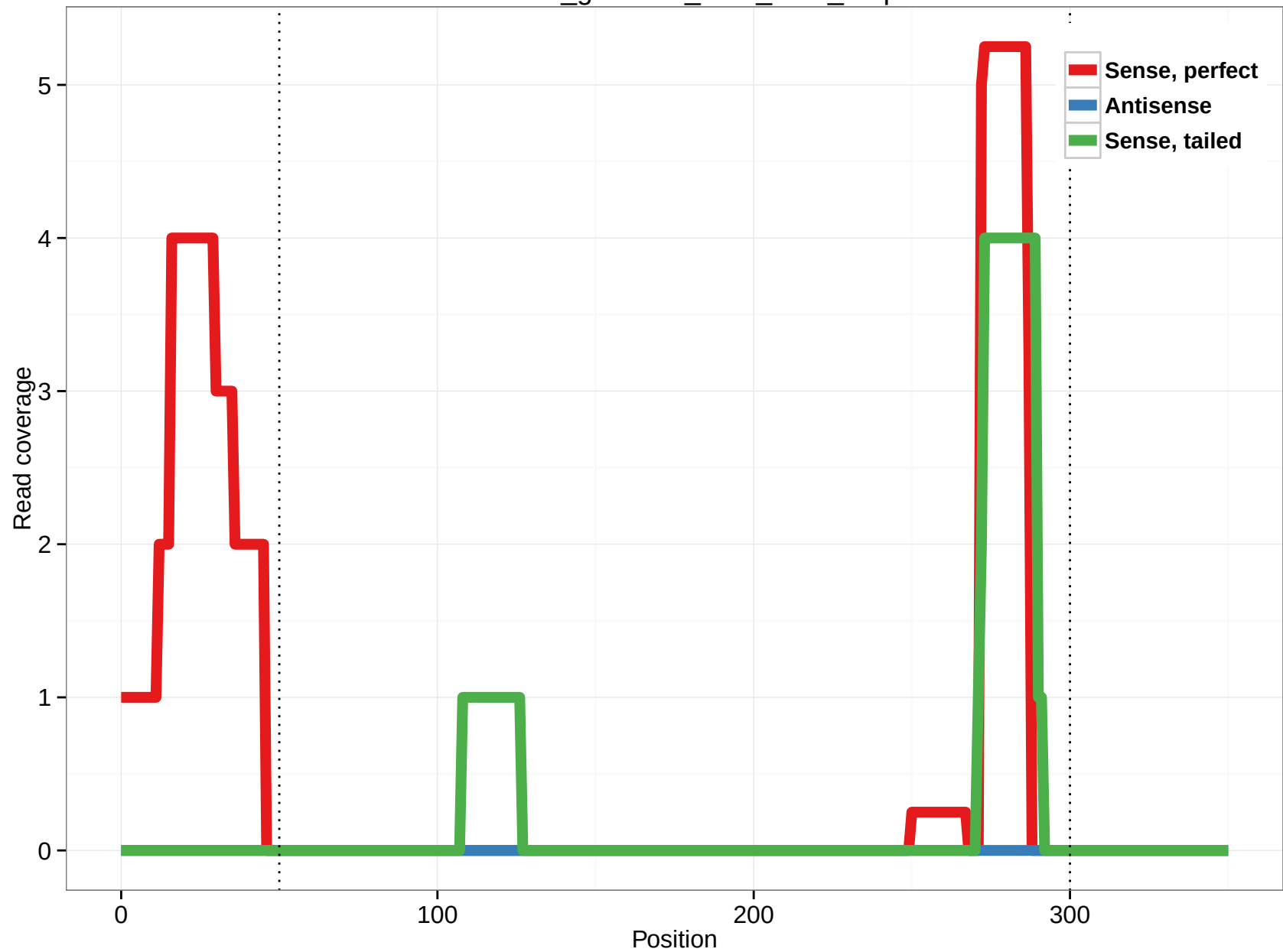
rheMac3_genscan_chr8_53.4_5.5p
