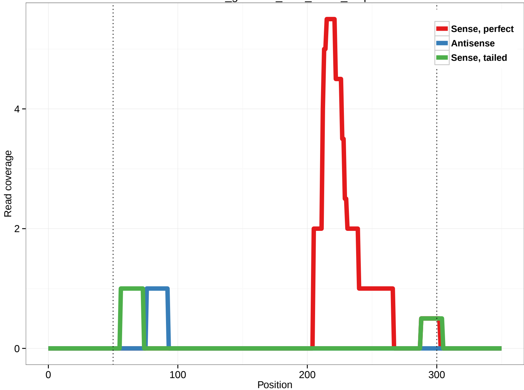
rheMac3_genscan_chr8_165.6_7.5p
