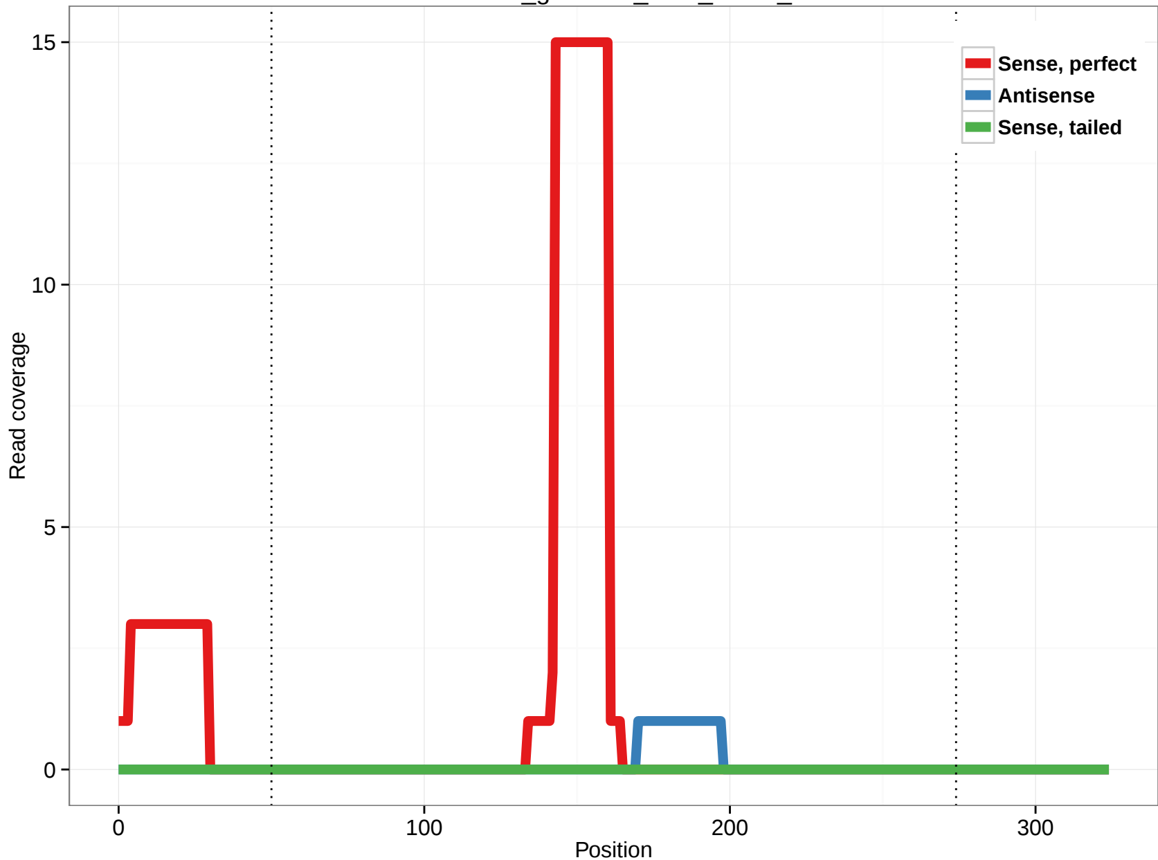
rheMac3_genscan_chr8_165.6_6
