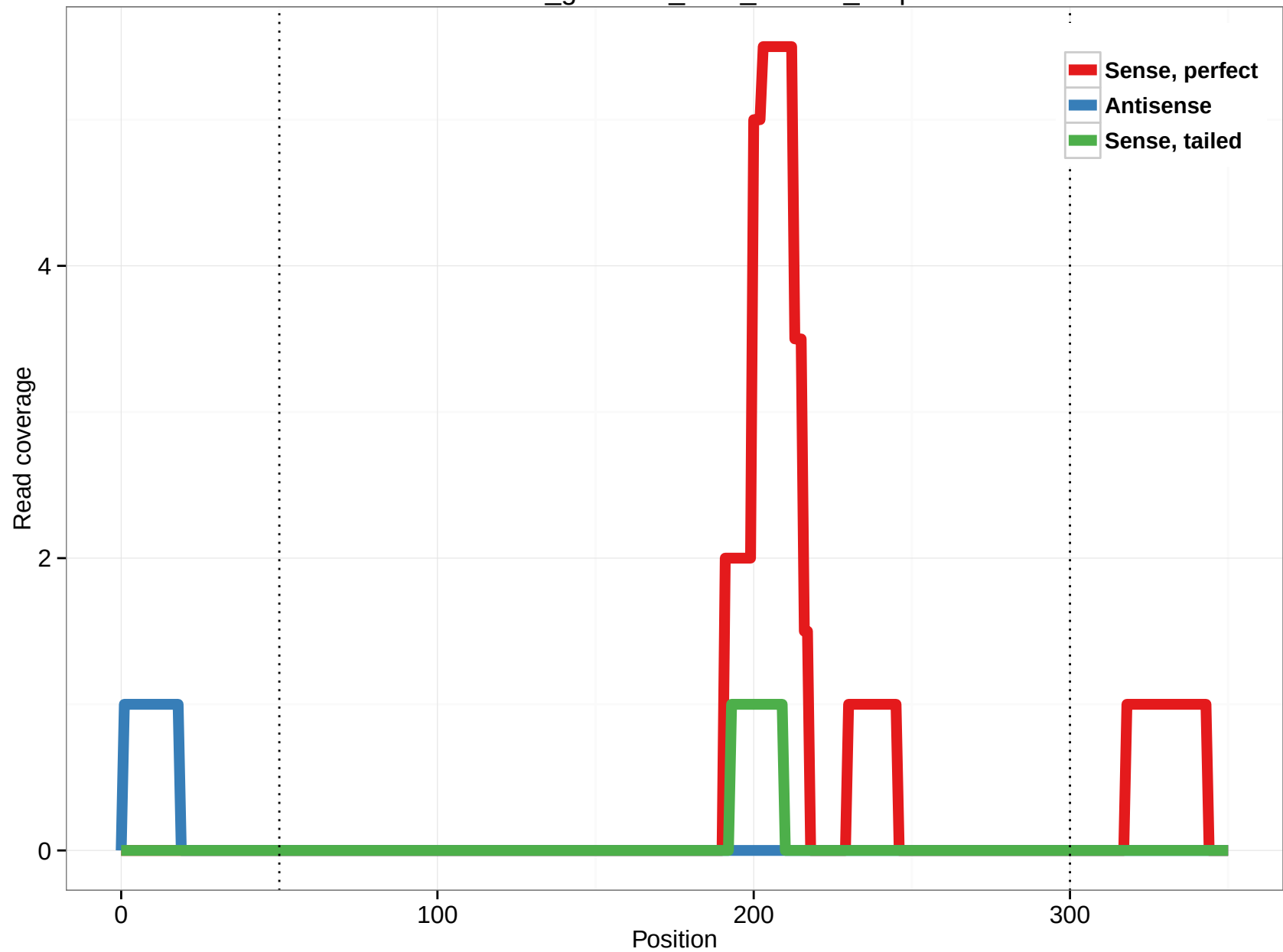
rheMac3_genscan_chr8_165.23_4.5p
