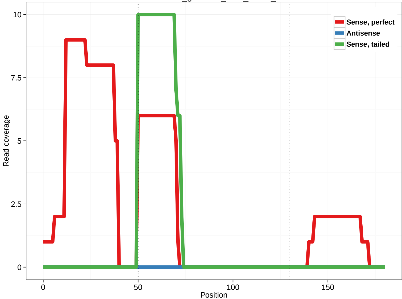
rheMac3_genscan_chr8_165.1_6
