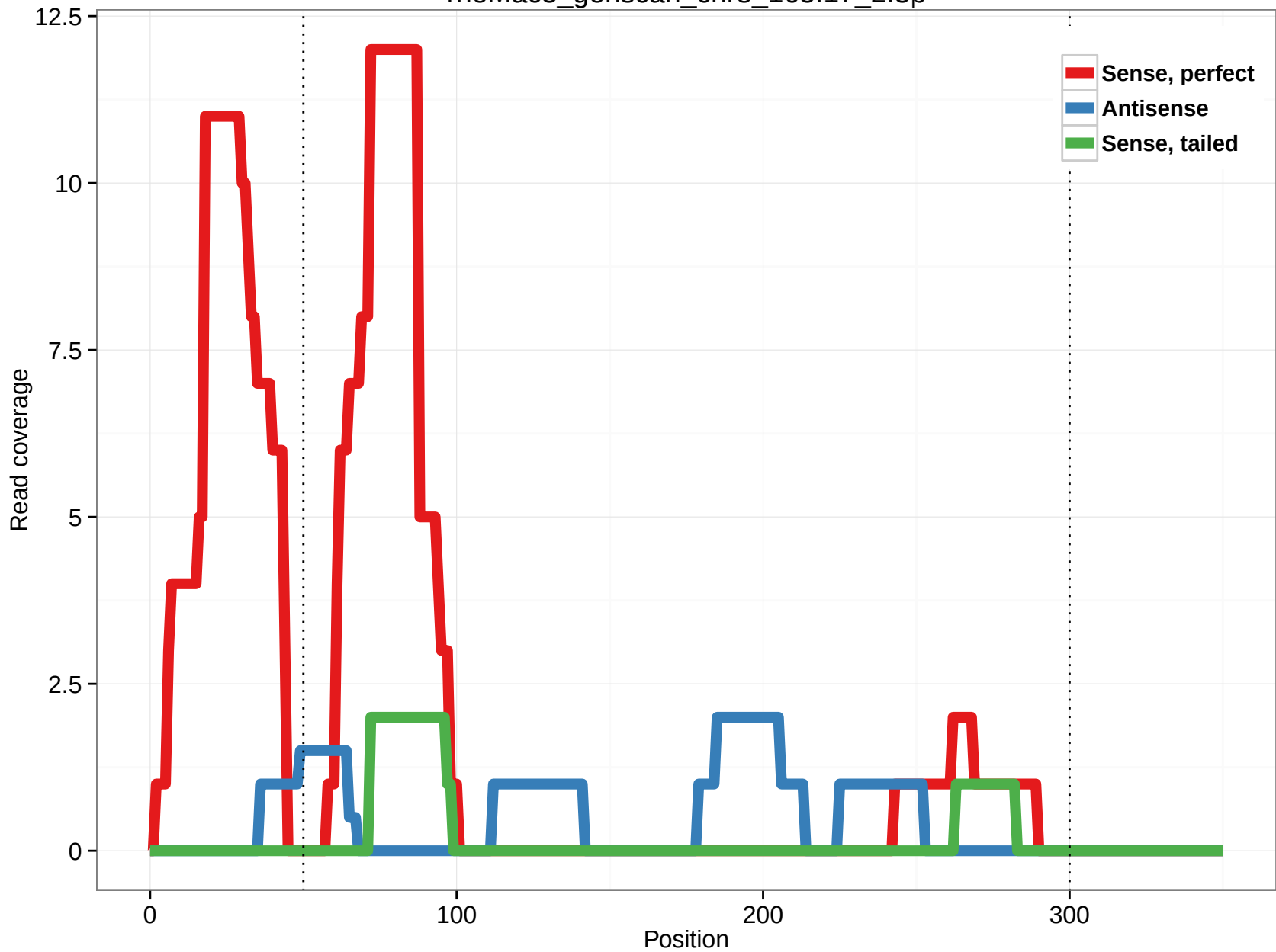
rheMac3_genscan_chr8_165.17_2.3p
